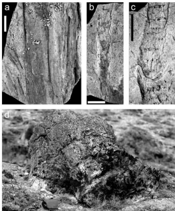
Figure 4. Typical elements of the permineralized and compression flora in the Chon Aike Formation – Tobas de Caída El Fénix Tufts (CAT). (a) Decorticated branch. Scale bar: 1 cm. (b) Brachyphyllum sp. branch with poorly preserved scale leaves. Scale bar: 1 cm. (c) Sphenophyte stem with whorled leaf scars. Scale bar: 1 cm. (d) Permineralized stump (about 1.5 m diameter) in growth-position on inclined substrate. Largest of the massive lateral roots (about 1 m diameter) points downhill towards bottom right of image.
