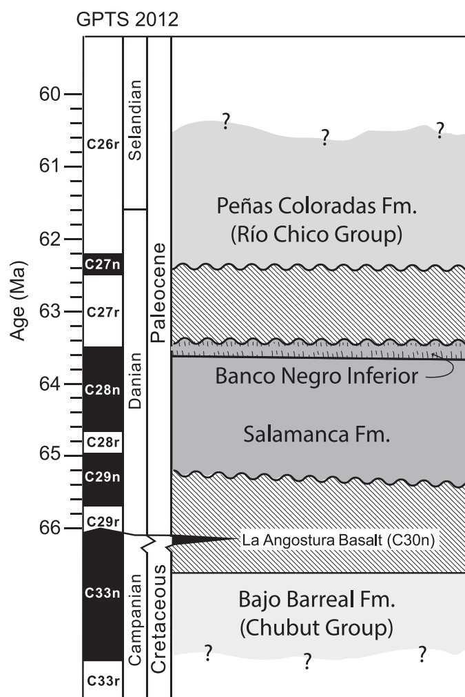
FIG. 2.—Generalized chronostratigraphy of latest Cretaceous and Paleocene geological units within the study area of the north-central San Jorge Basin, based on descriptions by Feruglio (1949), Uliana and Biddle (1988), Sylwan (2001), Raigemborn (2006), Iglesias (2007), Raigemborn et al. (2009), Krause and Piña (2012), and new age data in Clyde et al. (2014). Cross-hatch = section missing from non-deposition or erosion.
