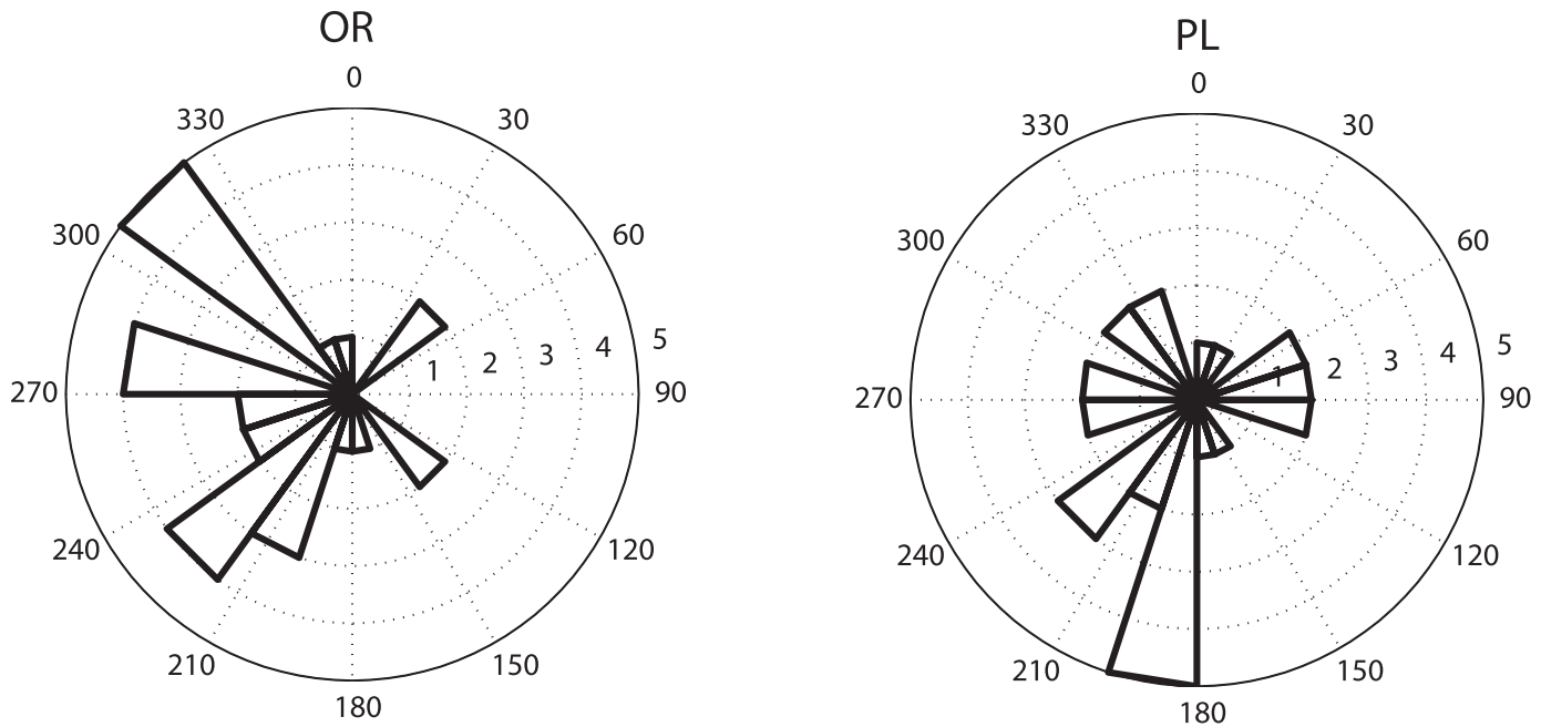
FIG. 6.—Rose diagrams showing paleocurrent directions of facies S_{wc} at Ormachea Park (OR, left) and Palacio de los Loros (PL, right). Zero degrees = True North. Paleocurrents cluster to the NW and SW.
