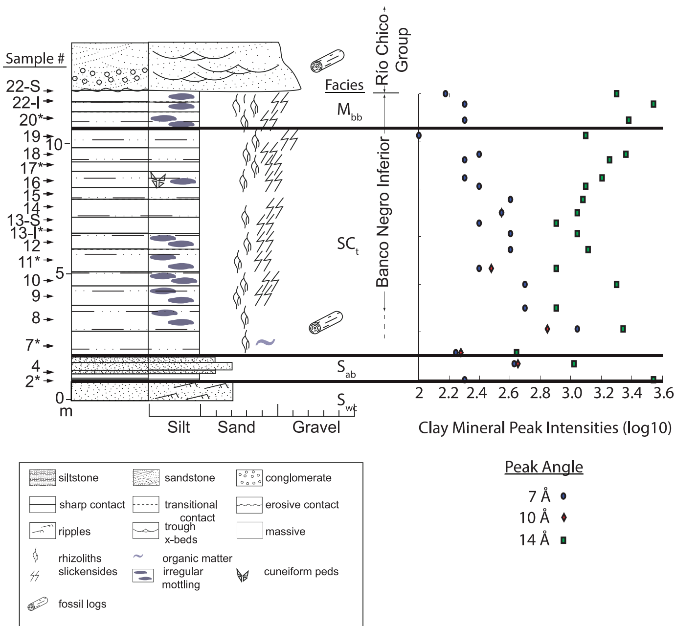
FIG. 3.—Graphic log from cliff face adjacent to plant locality OR-1 (denoted by star in locality inset map of Figure 4A), showing stratigraphic locations of XRD and chemical analysis samples. Samples used in the chemical analyses are 2, 7, 11, 13-I, 17, and 20 (denoted by asterisks). Facies definitions summarized in Table 1. Clay mineral peaks are interpreted as: 7 Å = kaolin-mineral; 10 Å = illite/glaucanite; and 14 Å = smectite. Intensity of the 7 Å peak shows a general decline upwards.
