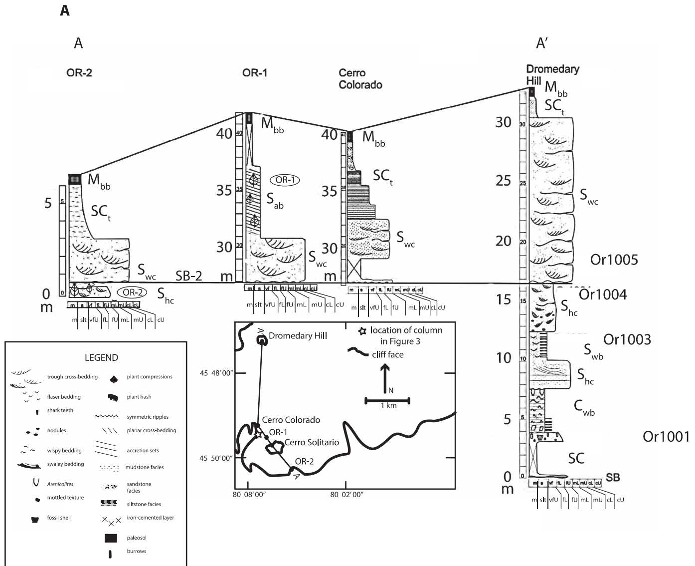
FIG. 4.—Selected graphic logs. A) Ormachea Park. B) Palacio de los Loros. Datum is an erosion surface defined as a sequence boundary (SB-2). Annotations refer to facies types in Table 1; OR1001 to OR1005 represent locations of samples for sand petrography; ellipses OR-1, PL-1, etc. denote macrofloral fossiliferous horizons.
