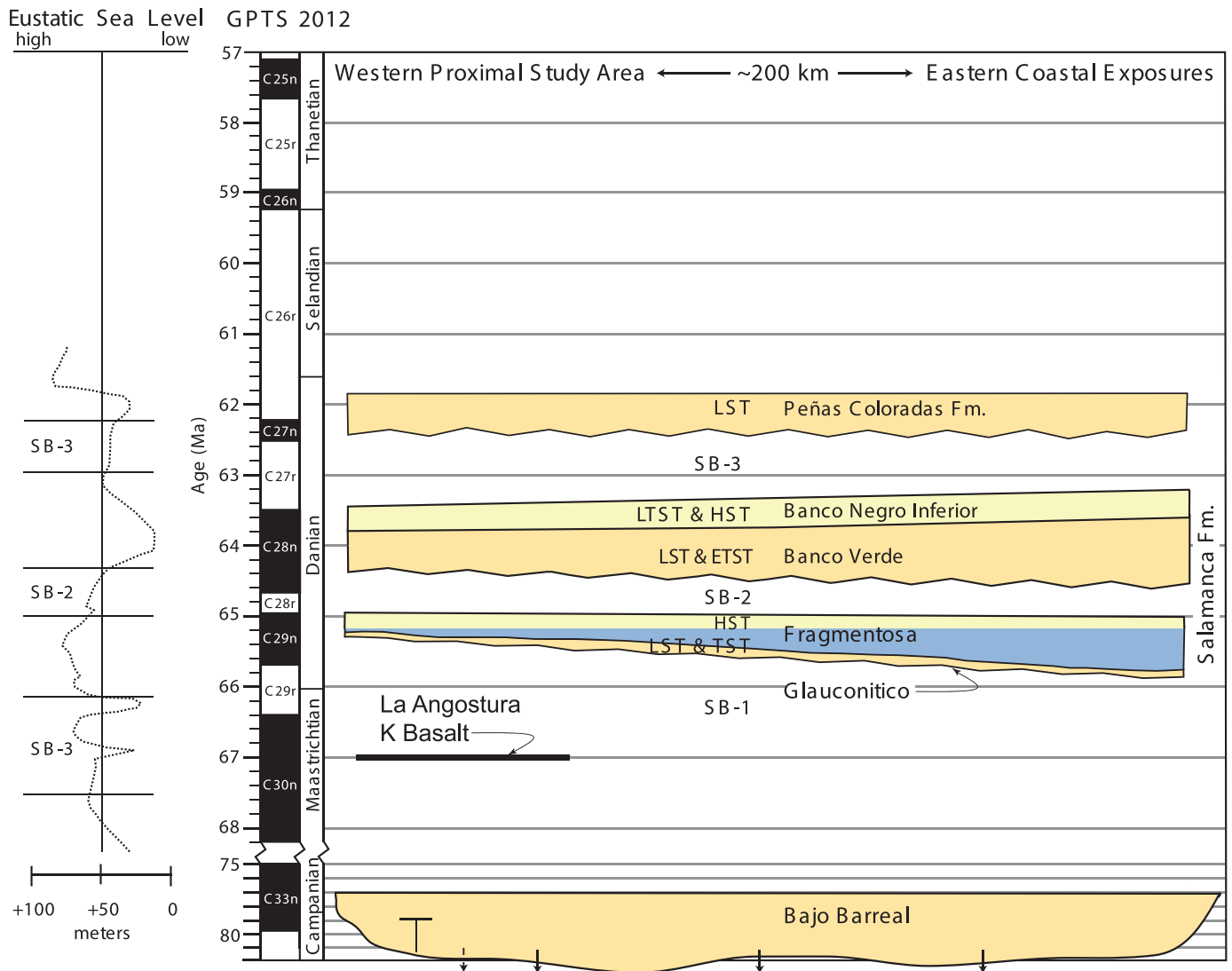
FIG. 8.—Wheeler diagram of stratigraphic events in the study area during the late Cretaceous through early Paleocene, modified from Clyde et al. (2014). Eustatic sea level curve from Kominz et al. (2008). Salamanca facies names after Feruglio (1949) and Bond et al. (1995). The basalt that lies between the Bajo Barreal and Salamanca formations is ^{40}\text{Ar} - ^{39}\text{Ar} dated to 67.31 \pm 0.55 Ma, and a tuff in the Peñas Coloradas Fm. at PL is U-Pb dated to 61.984 \pm 0.041 (Clyde et al. 2014). SB = sequence boundary; LST = lowstand systems tract; TST = transgressive systems tract; HST = highstand systems tract; (E or L)TST = early or late transgressive systems tract, respectively.
