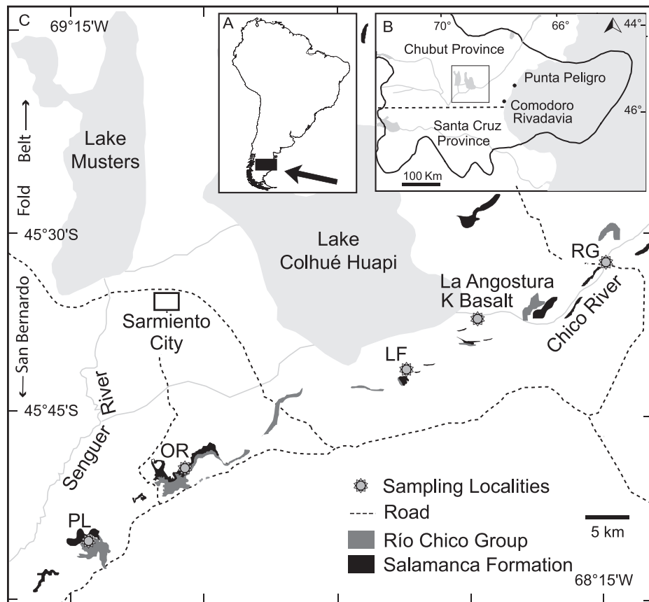
FIG. 1.—Map showing the San Jorge Basin and relevant localities (modified from Clyde et al. 2014). A) Location of study area. B) Boundary of the San Jorge Basin (solid line) as described by Sylwan (2001); gray represents lakes and rivers. C) Salamanca Fm. outcrops in black and Río Chico Group in dark gray (Brea et al. 2005; Iglesias 2007). The dashed lines represent major highways 20 and 26 in the area. Sampling localities: PL = Palacio de los Loros; OR = Ormachea Park; LF = Las Flores; RG = Rancho Grande.
