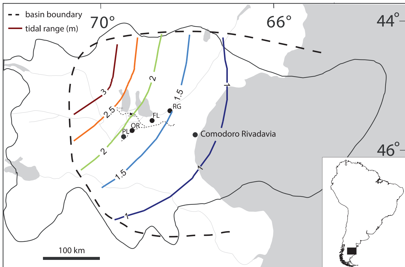
FIG. 10.—Modeled tidal range for the San Jorge Basin with an arcuate boundary and water depths decreasing landward from 150 m to 3 m. See text for details. A 1 m tide in the open proto-Atlantic amplifies to 3+ m in the embayment. Locality abbreviations given in Figure 1.
