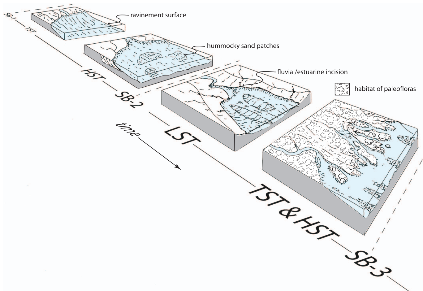
FIG. 11.—Schematic depositional model for the Salamanca Fm. in the study area. Abbreviations: SB = sequence boundary; TST = transgressive systems tract; HST = highstand systems tract; LST = lowstand systems tract. Detailed chronology of systems tracts given in Figure 9. Plant remains occur in many of the settings shown here; the superior preservation found at locality PL-2 corresponds to the legend item “habitat of paleofloras”.
