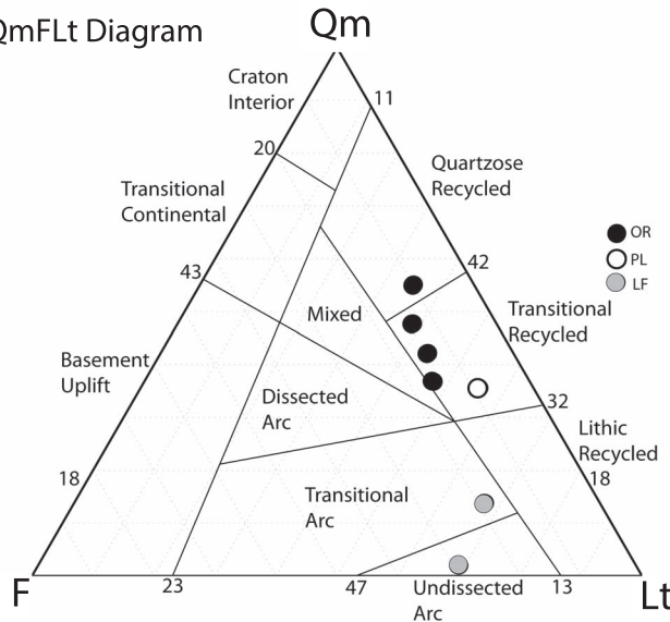
FIG. 9.—QFL and QmFLt diagrams of samples collected at PL, OR, and LF. A) QFL diagram based on the Dickinson et al. (1983) classification system; PL and OR samples lie within the recycled orogen domain, whereas LF samples lie within the undissected arc orogen domain. B) QmFLt diagram based on the Dickinson et al. (1983) classification system; PL and OR samples are classified as recycled orogen, whereas LF samples are classified as undissected arc and transitional arc orogens. Abbreviations: Q = total quartzose grains; F = monocrystalline feldspar grains; L = unstable polycrystalline lithic fragments of either igneous or sedimentary parentage, including metamorphic varieties; Qm = monocrystalline quartz; Lt = total polycrystalline lithic fragments including quartzose varieties.
