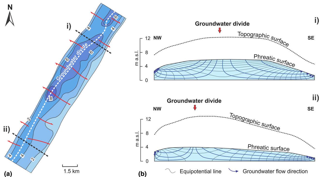
Fig. 6 a Groundwater contour map (Date: May 2014), the arrows indicate groundwater flow direction. b Simplified cross sections (i) for bare soil in the northern sector and (ii) for forested soil in the southern sector
