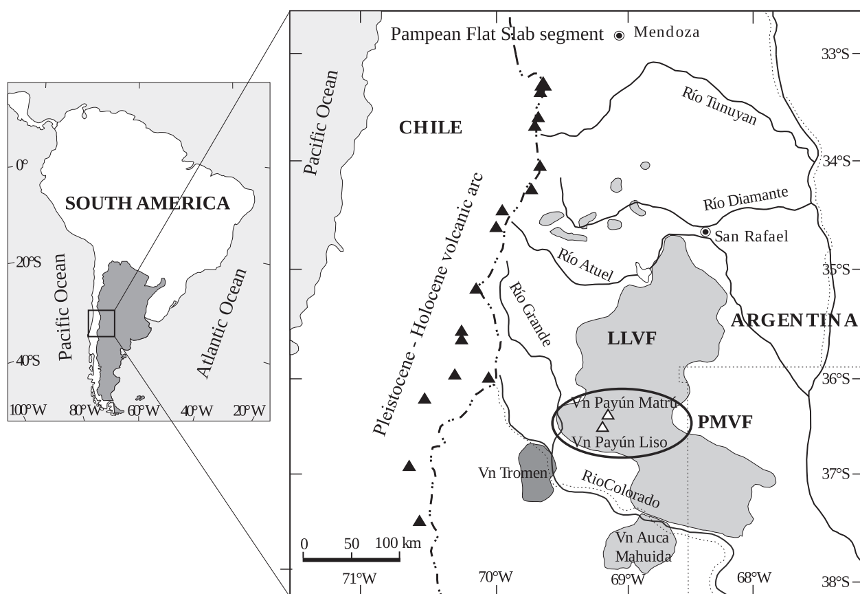
Fig. 1. Location map of the Payenia Basaltic Province (light gray) in the back-arc of the Southern Volcanic Zone of the Andes and the Pleistocene–Holocene volcanic arc (black triangles). The Tromen volcanic complex (dark gray) is not generally considered as part of Payenia. The oval indicates the location of the Payún Matrú Volcanic Field (PMVF). LLVF, Llancanelo Volcanic Field.
