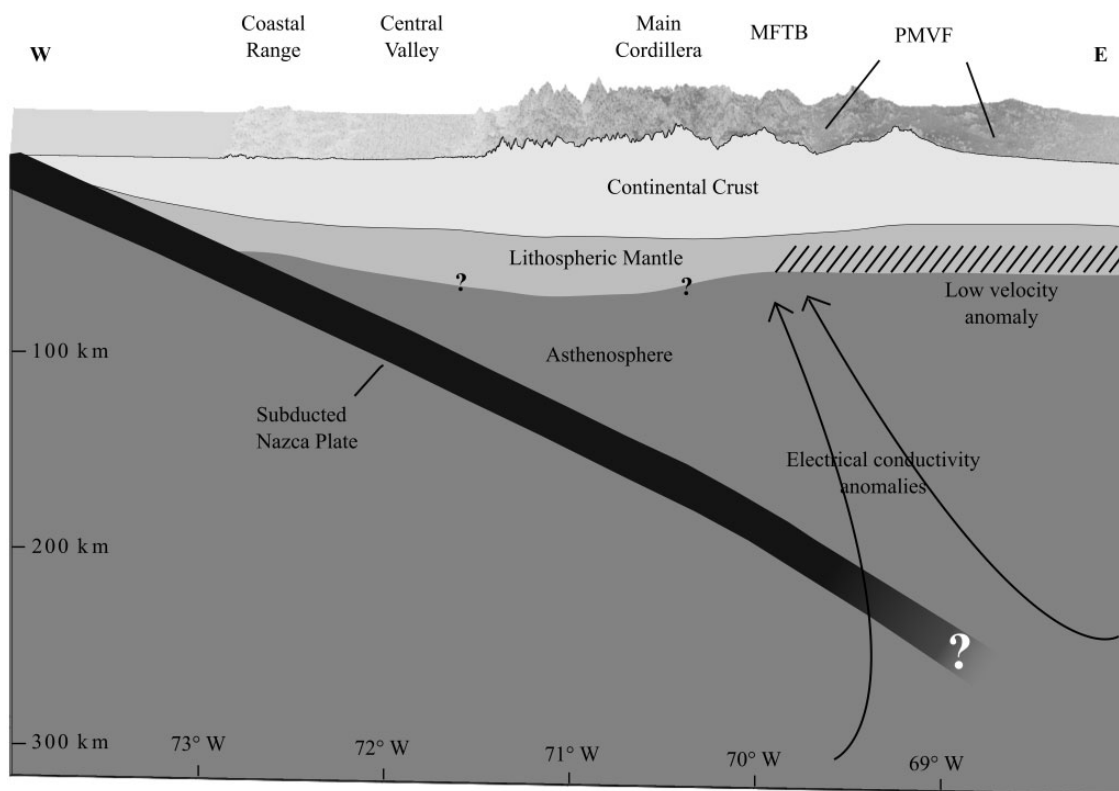
Fig. 18. Schematic west-east profile of the western margin of South America at 36°25'S with topographic vertical exaggeration of around six. The subducted Nazca plate has been drawn according to the mantle profile shown in Fig. 17a, where it is observed that the slab could be interrupted to the east of the PMVF, as indicated by the question mark. The thickness of crust and mantle in the arc and back-arc zone are as inferred by Wagner et al. (2005) and Gilbert et al. (2006). The diagonally shaded zone corresponds to seismic anomalies in the back-arc area, with a zone of low velocity between 40 and 60 km depth, interpreted as the possible base of the lithosphere (Gilbert et al. , 2006). Arrows show the schematic position of electrical conductivity anomalies below the PMVF (Burd et al. , 2008). MFTB, Malargüe fold and thrust belt (Miocene).
