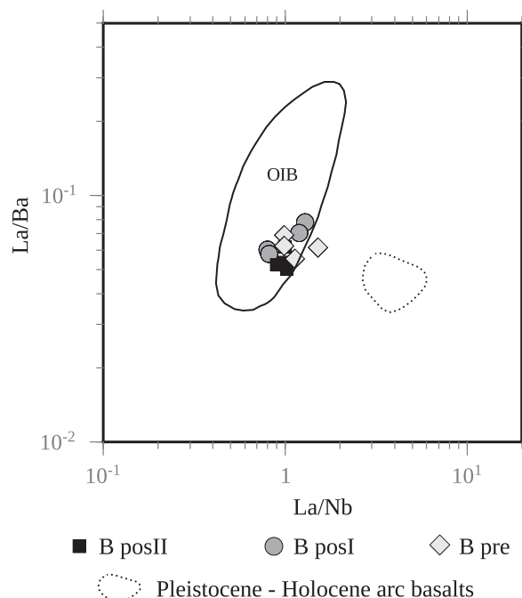
Fig. 12. \text{La}/\text{Nb} vs \text{La}/\text{Ba} for basalts and trachybasalts of the PMVF (after Fitton et al. , 1991), and basalts of the Pleistocene-Holocene volcanic arc (field with dotted outline) (Tormey et al. , 1991). The OIB field is based on more than 900 analyses of OIB from various ocean islands (Fitton et al. , 1991).
