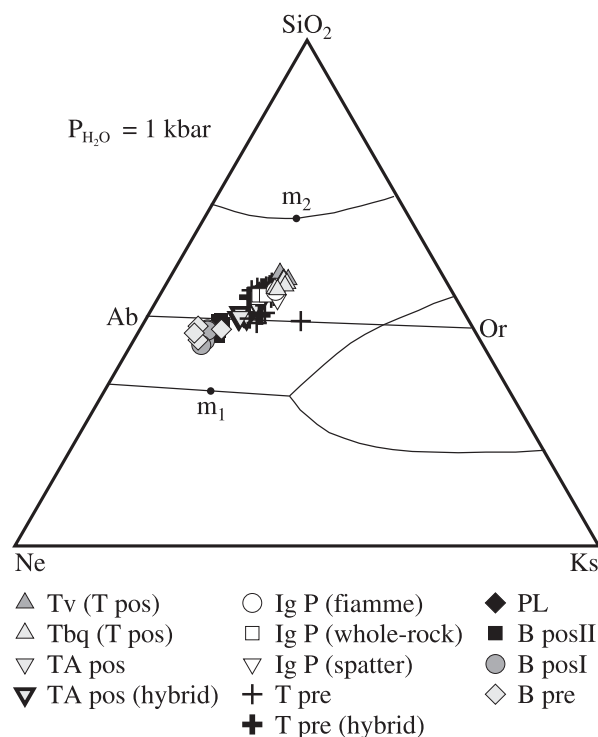
Fig. 16. \text{SiO}_2\text{--NaAlSi}_3\text{O}_4 (Ne)– \text{KAlSi}_3\text{O}_4 (Ks) residual system showing all samples of the PMVF. Phase boundaries ( P_{\text{H}_2\text{O}} 1 kbar) according to Hamilton & MacKenzie (1965). m_1 , silica-undersaturated thermal minimum; m_2 , silica-oversaturated thermal minimum. Although this diagram is traditionally used for silicic compositions, here the basalts are also plotted to illustrate the characteristics of the whole volcanic field. Because mafic minerals are an important component of basaltic magmas, the residual system does not fully represent these magmas. The general evolutionary trend of Payún Matrú rocks is towards the silica-oversaturated thermal minimum.
