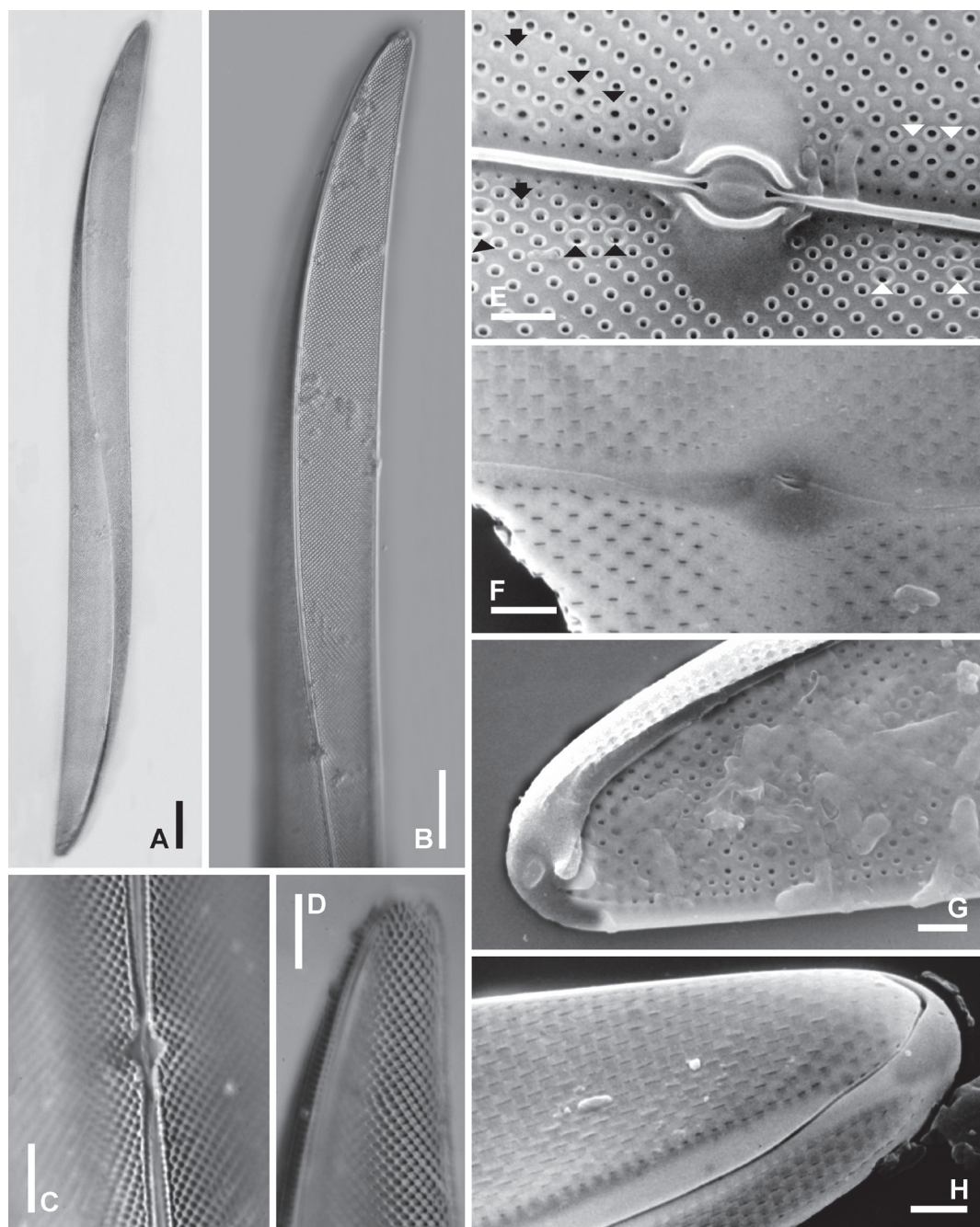
Fig. 1. Pleurosigma formosum , type material. LM: A-D, SEM: E-H. A: Valve linear, sigmoid. B: Detail of A showing central area and terminal areas unilaterally dilated, funnel shaped, in apical position. C: Central area circular. D: Detail of an apex showing striation pattern. E, G: Internal views. F, H: External views. E: Central area saddle shaped with central bars surrounding the circular, central nodule. Note circular, rimmed, hymen-occluded pore, crossed by a recessed bar (arrows) and pairs of pores more deeply recessed in the siliceous layer and lacking the central bar (arrowheads). F: Detail of a valve showing central raphe fissures. G: Polar ending terminating in helictoglossa. H: Apex showing terminal raphe fissure hook-shaped. Scale bars: A-B, 25 \mu m; C-D, 5 \mu m; E-H, 2 \mu m.
