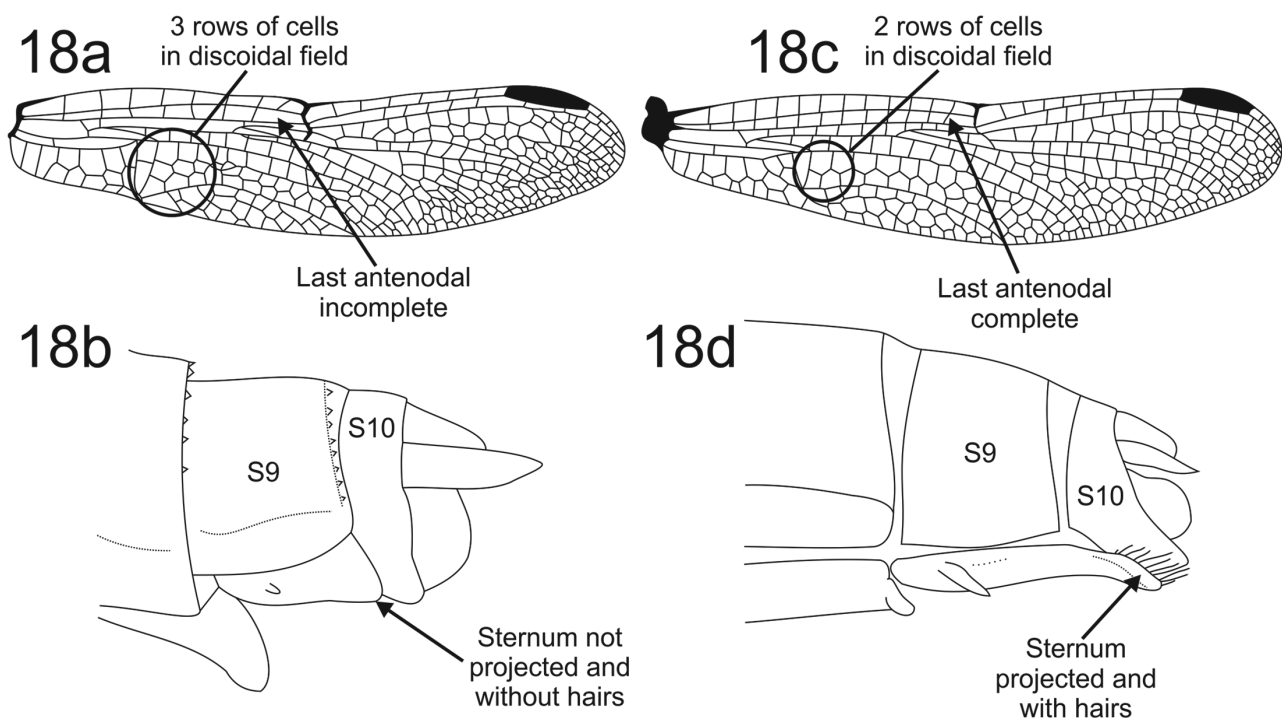
FIGURE 18. a Sympetrum villosum , Fw showing vein characters (modified from Garrison et al. 2006); b Erythrodiplax nigricans , female terminalia, lateral view (modified from Borror 1942); c Dasythemis mincki clara , Fw showing vein characters, Fw showing vein characters (modified from von Ellenrieder & Garrison 2007); d Dasythemis mincki clara , female terminalia, lateral view (modified from von Ellenrieder & Garrison 2007).
