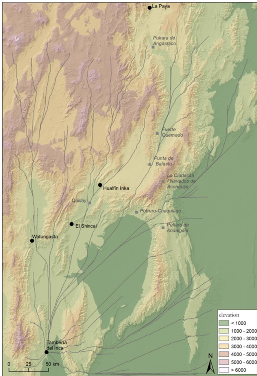
Fig. 5. Results of the MADO analysis towards Tambería del Inca.
