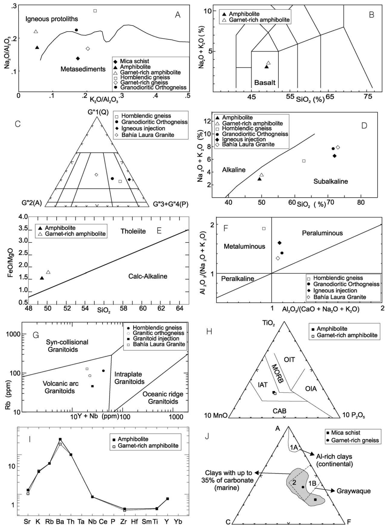
Fig. 4. Geochemical diagrams from the Bahia Laura metamorphic and igneous rocks. (A) Garrels and Mackenzie, 1971; (B) Le Maitre, 1989; (C) La Roche, 1992; (D) Irvine and Baragar, 1971; (E) Miyashiro, 1974; (F) Maniar and Piccoli, 1989; (G) Pearce et al., 1984; (H) Pearce and Norry, 1979; (I) MORB after Pearce, 1981; and (J) Winkler, 1978.
