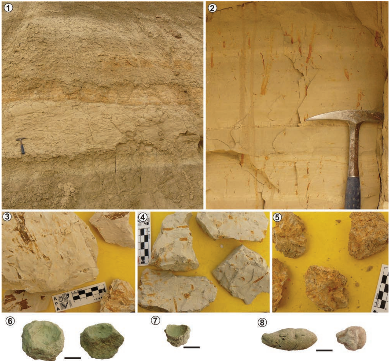
Figure 2. Different features of Facies Association 1 deposits. 1, succession of structureless strata composed of pedogenically-modified fine tuffaceous sandstones and mudstones. 2, Detail of laminated siltstones and mudstones with different types of orange-colored root traces. 3, Plant remains preserved on lamination planes of mudstone. 4, Detail of angular to subangular blocky pedes with ferric delicate and haloed root traces. 5, Detail of subangular blocky to granular pedes with abundant root traces and mottles. 6, Fragments of Coprinisphaera isp. 7, Feoichnus challa . 8, Coprolites. Scale bars for 6, 7 and 8 = 1 cm.
