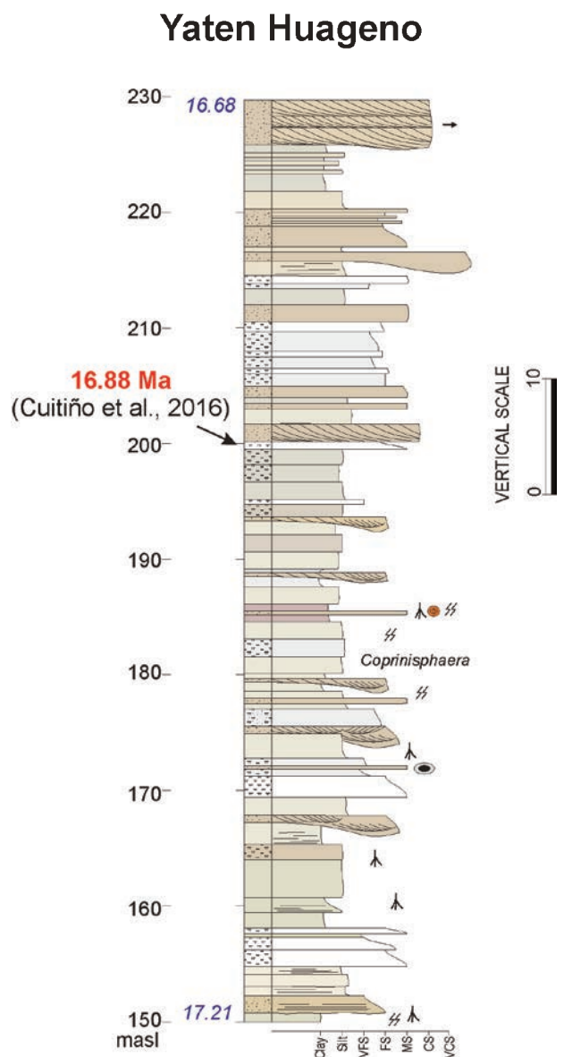
Figure 13. Sedimentary section measured for Yaten Huageno locality showing the dated horizon. The red number indicates the U/Pb age whereas the blue numbers are estimated upon sedimentation rates. For references see Figure 8.
