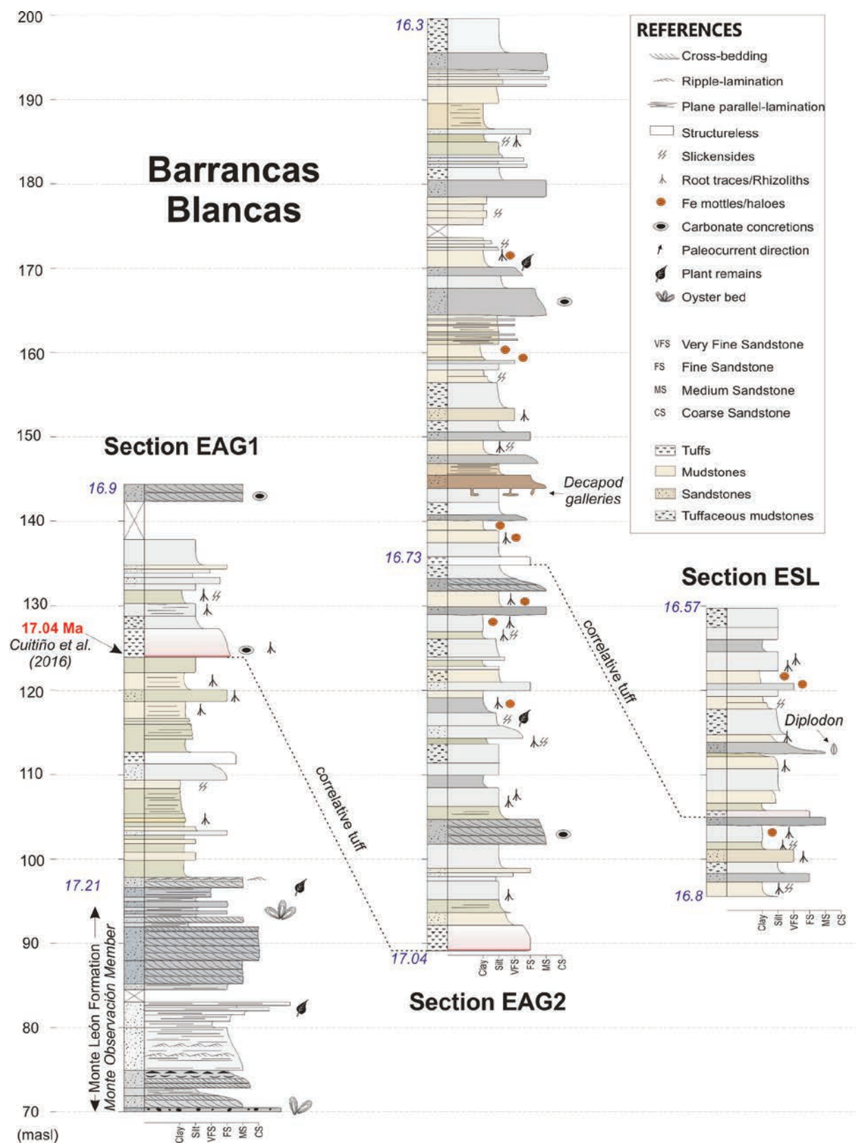
Figure 8. Sedimentary sections measured in Barrancas Blancas locality, showing local correlative horizons. The red number indicates the position of the U-Pb age (Cuitiño et al. , 2016) whereas the blue numbers are ages estimated upon sedimentation rates.
