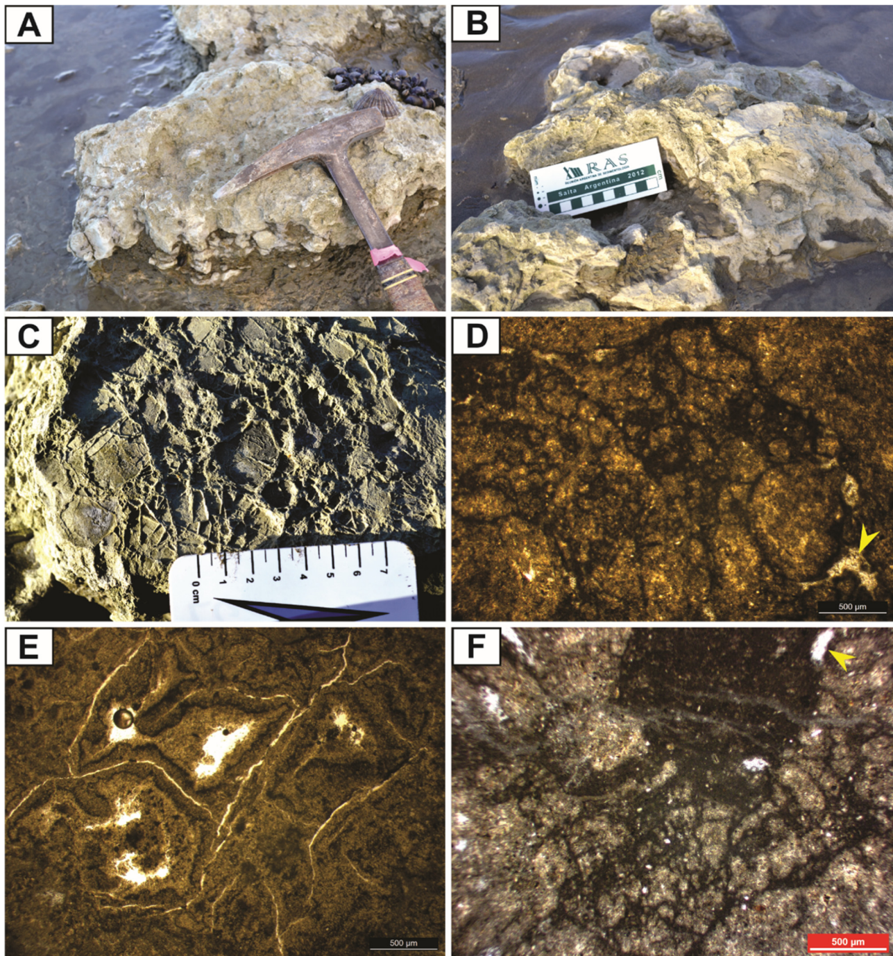
Fig. 6. Macro- (A–C) and micromorphological (D–F) features of the massive-calcretes (M-calcrete). A and B., Crust-like morphology in the current intertidal setting. C., Network of cracks in the upper surface of the massive-calcretes. D., Peloidal aspect of the micritic groundmass and microspar cements (arrow) (NX, x4). E., Empty micro-desiccation cracks (NX, x4). F., Mottling aspect and microspar cement (arrow) (NX, x4).
