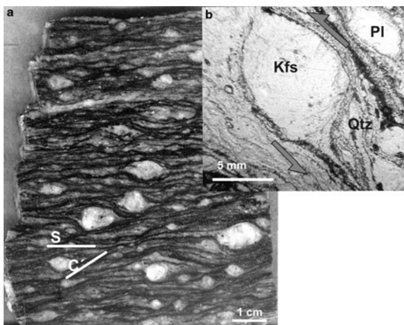
Fig. 2 (a) Mylonitic texture of SPP-2007 orthogneiss with S-C' composite foliations (section parallel to L_{myl} ). (b) Asymmetric Kfs porphyroclasts in a fine-grained groundmass of dynamically recrystallized quartz and biotite.
