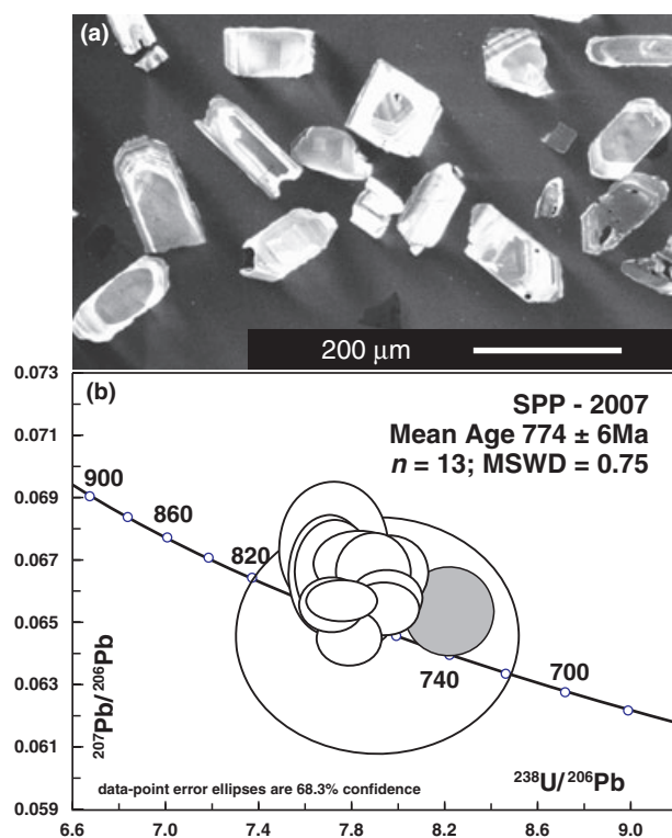
Fig. 4 (a) Cathodo-luminescence images of SPP-2007 zircons showing unzoned cores, magmatic oscillatory-zoned overgrowths and a thin luminescent rim. (b) Tera-Wasserburg diagram of the full dataset showing error ellipses at 68.3% confidence limits for igneous cores and rims.
