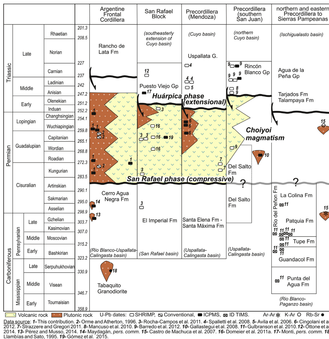
Fig. 2. Late Paleozoic to Triassic tectonomagmatic evolution and age constraints for the Choiyoi magmatism in Argentine Frontal Cordillera, San Rafael Block and part of the Argentine Precordillera to Sierras Pampeanas between 28° and 35°S. See Fig. 1 for location of morphostructural provinces. The early Permian San Rafael compressive phase affects the Carboniferous to earliest Permian strata in the Rio Blanco–Uspallata–Calingasta and San Rafael basins and marks the initiation of the Choiyoi magmatism. The effect of the San Rafael phase seems to be uncertain in the Paganzo basin of Sierras Pampeanas region. The end of the Choiyoi magmatism is marked by a generalized extensional event (Huárpica phase) that causes the rift stage during the Triassic. In this way, the Choiyoi magmatism in this region is constrained between the Cisuralian and Early Triassic. Stratigraphically below and above, magmatism is found mostly interlayered in sedimentary sequences, as tuffs, pyroclastic flows and lavas, and in minor degree, as intrusive bodies. Time Scale used: International Chronostratigraphic Chart v2014/02.
