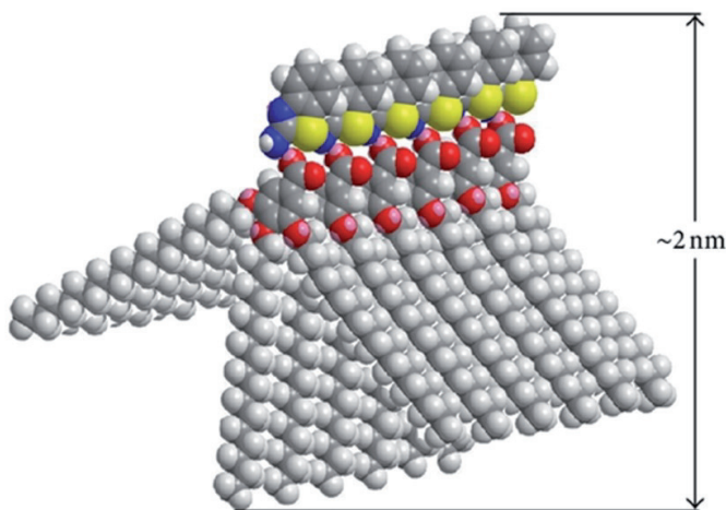
Figure 22. A reasonable self-assembly mode for S-TriC18 organogels.
