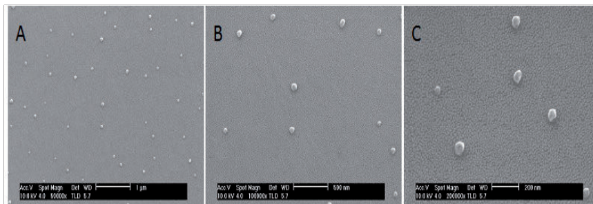
Figure 1. The films of SWNHs40/PS observed by SEM. SWNHs40-coated PS (0.85 \mu\text{g}/\text{cm}^2 ) dishes with a bottom area of about 1 \text{cm}^2 were prepared for SEM measurements. After pretreated by spraying gold on films of samples, SEM measurements were carried out using a SIRION field emission scanning electronic microscope (FEI Corporation Ltd) with accelerating voltage of 10.0kV. The SEM of films showed that SWNHs40 on PS surface (0.85 \mu\text{g}/\text{cm}^2 ) were individual spherical particles with diameters of 60-100nm. (A) 50,000 \times , scale bar represents 1 \mu\text{m} . (B) 100,000 \times , scale bar represents 500 nm. (C) 200,000 \times , scale bar represents 200nm.
