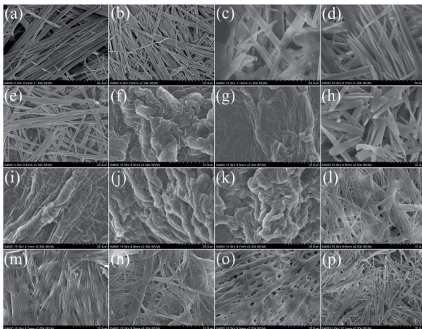
Figure 17. SEM images of xerogels. CH-C1 gels ((a) isoctanol, (b) n-hexane, (c) 1,4-dioxane, (d) nitrobenzene, (e) aniline), CH-C3 gels ((f) cyclohexanone, (g) 1,4-dioxane, (h) nitrobenzene, (i) ethyl acetate, (j) petroleum ether, (k) DMF), CH-C4 gels ((l) nitrobenzene, (m) aniline, (n) n-butyl acrylate, (o) DMF), and CH-N1 gels ((p) pyridine).
