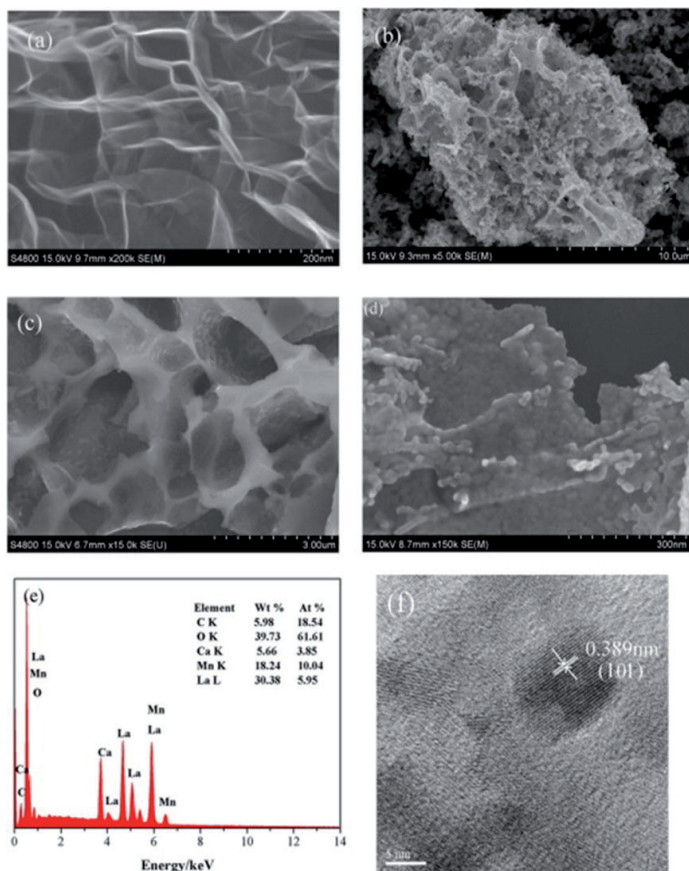
Figure 11. FESEM images of (a) graphene; (b, c, d) FE-SEM, (e) EDS, (f) HRTEM of \text{La}_{0.6}\text{Ca}_{0.4}\text{MnO}_3 -graphene composite.
