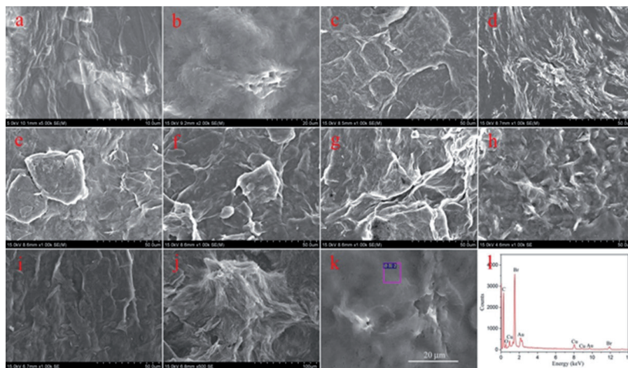
Figure 24. SEM images of xerogels. GO powder (a), C18-6-GO gels ((b) DMF), C18-12-GO gels ((c) DMF, (d) benzene, (e) toluene, (f) 1,4-dioxane, and (g) THF), and C18-6-18-GO gels ((h) cyclohexanone, (i) THF, and (j) pyridine). Typical EDXS (l) of xerogels originate from C18-6-GO gels in DMF (k). The Cu and Au peaks originate from the substrate of copper foil and the coated gold nanoparticles.
