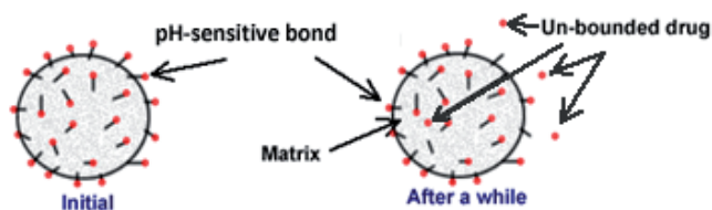
Scheme 4. Schematic representation of the delivery mechanism in pH-sensitive mechanism
