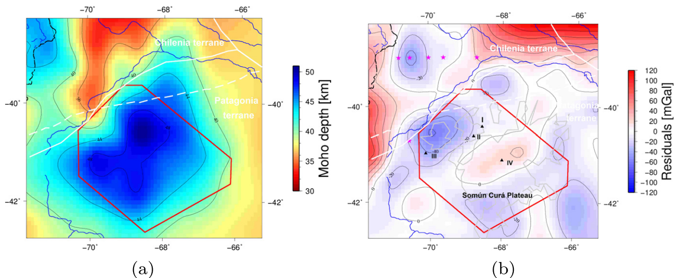
Fig. 6. Moho and residuals of the final model. The discontinuity between terranes from Chericoff and Zappettini (2004) is shown with white solid lines and the discontinuity in the velocity distribution with a dash line. a) Resulting Moho depth. b) Gravity residuals of the resulting model. The location of the constraining independent Moho depth data is shown with red stars. The outcropping basalts of the area are delimited in grey. The location of the xenolith samples are shown with black triangles.
