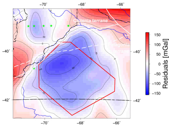
Fig. 5. Gravity residuals of the initial model. The location of the constraining independent Moho depth data is shown with green stars. The discontinuity between terranes from Chericoff and Zappettini (2004) is shown with white solid lines, and the S-wave velocity constrained boundary between terranes in a white dash line.
