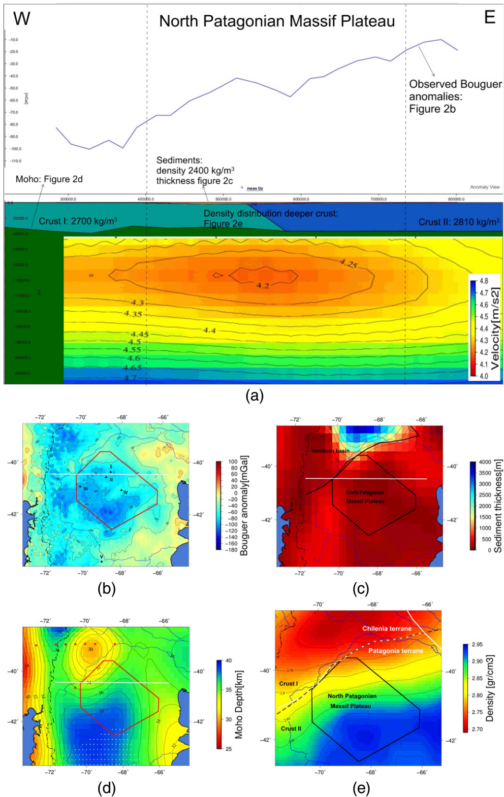
Fig. 2. Initial density model. a) Schematic profile showing a cross section of the initial model and the input data. The velocity distribution profile is from SL2013Sv model (Schaeffer and Lebedev, 2013). The location of the profile is shown in white in Fig. 2(b), (c) and (d). b) Bouguer anomalies from EGM2008 (Pavlis et al., 2012) used as measured gravity for the 3D density model. The localities where there are xenolith data (Ponce, 2016 and Mundl et al., 2015) are indicated by black triangles. I: Cerro Chenque, II: Puesto Diaz, III: Comallo, IV: Pahuaniyeu, V: Paso de Indios. c) Sediment thickness in the study area from Heine (2007). d) Moho depth of the initial model extracted from Assumpção et al. (2012). The area with white points has no resolution and was interpolated to be used in the initial model. The location of the Moho depth data from seismics are shown with red stars. e) Density configuration at 25 km depth, converted from SL2103Sv model (Schaeffer and Lebedev, 2013). The discontinuity between terranes from Chernicoff and Zappettini (2004) is shown with white solid lines. The final discontinuity between the two crustal bodies modelled is shown with black dashed line.
