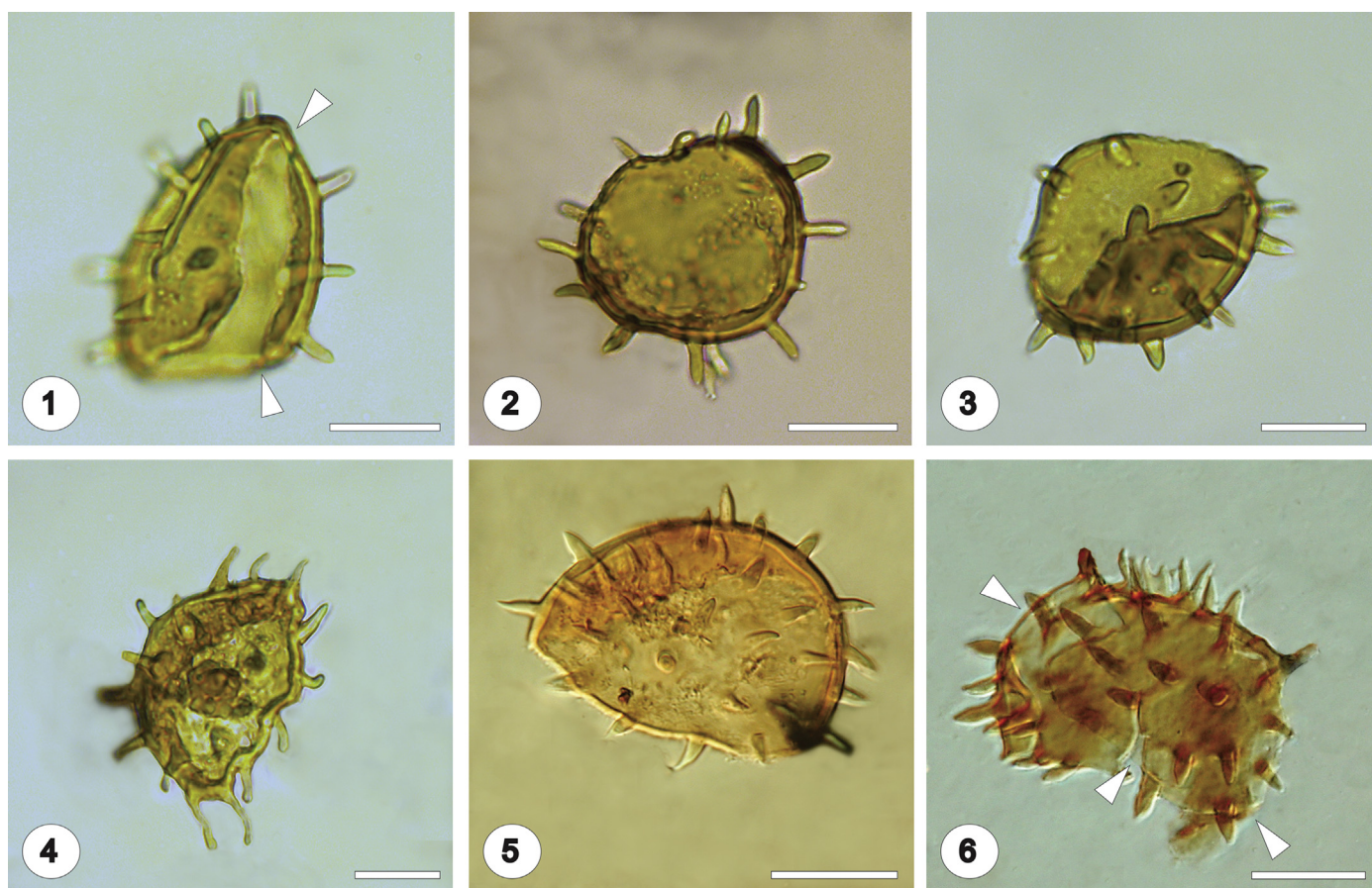
Fig. 5. Spinizonocolpites -type. Monads. All LM. All scales = 15 \mu m. 1-6. Monads showing spines and zonosulcus (white arrows). 1. BA Pal 6325. 2. BA Pal 6326. 3. BA Pal 6325. 4. BA Pal 6325. 5. BA Pal 5668. 6. Broken specimen showing spines and zonosulcus (white arrows), BA Pal 6292.
