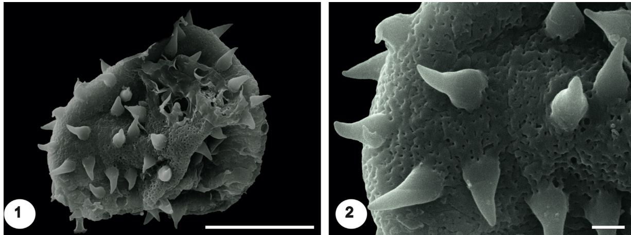
Fig. 6. Spinizonocolpites -type. Monad. All SEM. 1–2. BA Pb MEB 524. Monad. Scale = 10 \mu\text{m} . 2. Detail of perforate sculpture. Scale = 1 \mu\text{m} .
