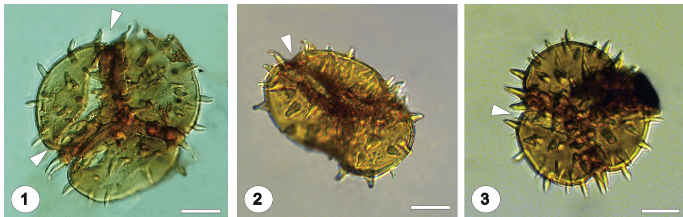
Fig. 4. Spinizonocolpites -type. Tetrads. All light microscope (LM). All scales = 15 \mu m. 1. Tetrahedral tetrad showing sulcus and supratergal spines. Zonosulcus (white arrows), BA Pal 5697.2-3. Tetrahedral tetrad. Zonosulcus (white arrows). 2. BA Pal 6327. 3. BA Pal 6325.
