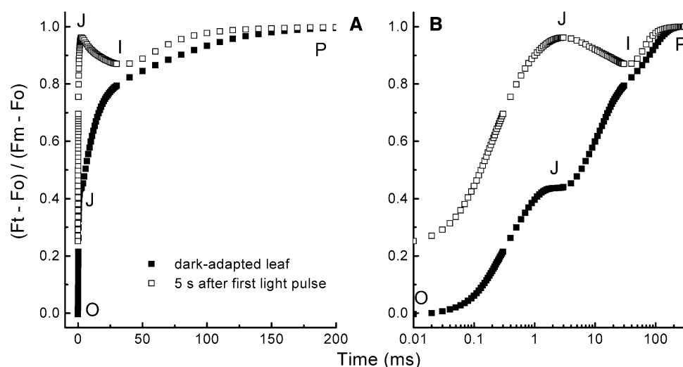
Fig. 3 OJIP transients (double normalized between O and P) measured on a bean leaf ( Phaseolus vulgaris ) shown on a linear timescale ( a ) and a logarithmic timescale ( b ). A measurement on dark adapted (closed symbols) which has an oxidized PQ-pool and a low J-step and a measurement made 5 s later (open symbols) where Q_A
