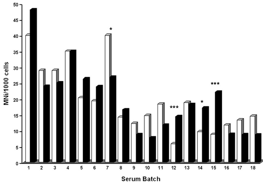
Fig. 2. Frequency of MNi in CHO-K1 cells cultured with different 18 commercial lots of FCS after \gamma -irradiation (white bars) and their non-irradiated counterparts (black bars). Each bar represents the mean number of MNi among 1000 cells scored per experimental point. *, P < 0.05 ; ***, P < 0.001 , significant differences between pairs of sera.
