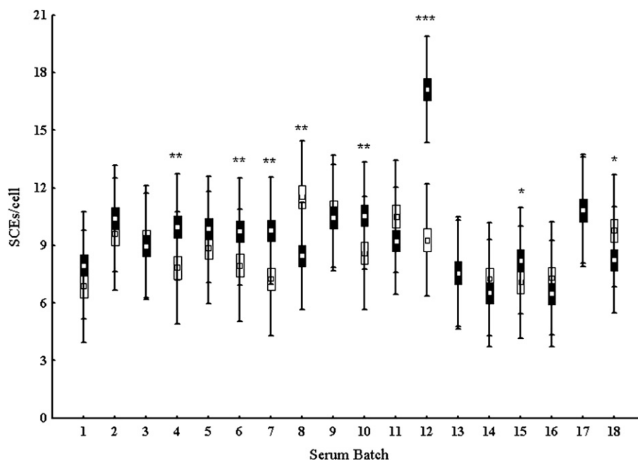
Fig. 1. Frequency of SCEs in CHO-K1 cells cultured with 18 commercial lots of FCS after \gamma -irradiation (white boxes) and their non-irradiated counterparts (black boxes). Data are displayed as box plots, where the y-axis shows the range data from 75 s mitoses analyzed per cell culture. Each box encloses the median value of SCEs/cell (small white square). The top and the bottom of the box mark the SCEs mean value \pm SE of the mean. The lines extending from the top and the bottom of each box mark the pooled SD of the mean. *, P < 0.05 ; **, P < 0.01 ; ***, P < 0.001 , significant differences between pairs of sera.
