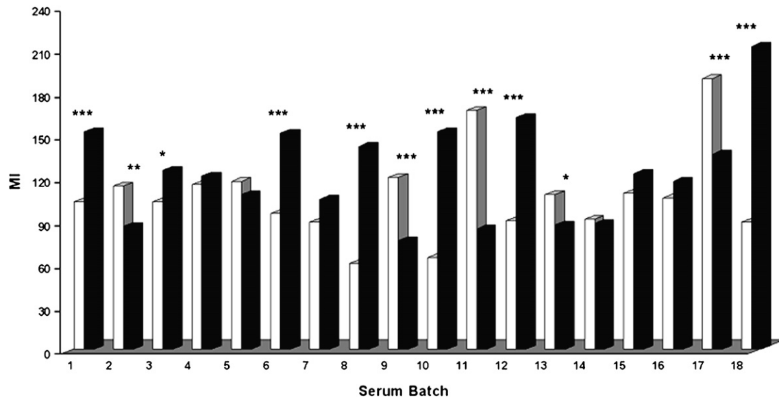
Fig. 3. Mitotic index analyses on CHO-K1 cells cultured with different 18 commercial lots of FCS after \gamma -irradiation (white bars) and their non-irradiated counterparts (black bars). Each bar represents the mean number of mitotic cells among 1000 cells scored per experimental point. *, P < 0.05 ; **, P < 0.01 ; ***, P < 0.001 , significant differences between pairs of sera.
