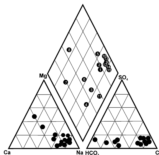
Fig. 5 Piper diagram for groundwater
