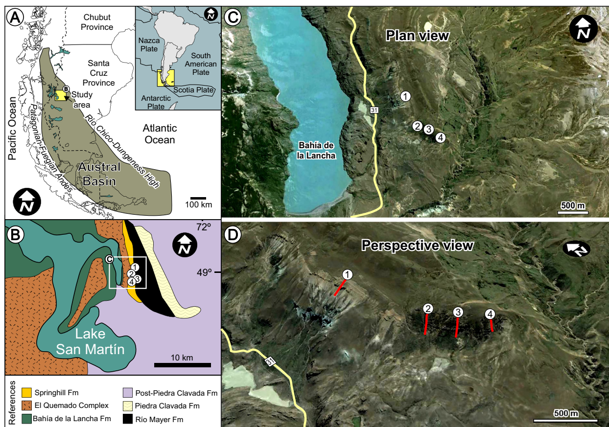
Fig. 1. Location of the Austral Basin in South America and position of the sedimentary logs in the study area. A, position of the Austral Basin in Argentina (South America). B, detailed geological map of the Lago San Martín locality and the sedimentary logs position. C, satellite image of the Bahía de la Lancha area and location of the four sedimentary sections analysed. D, perspective view of the deposits studied.
