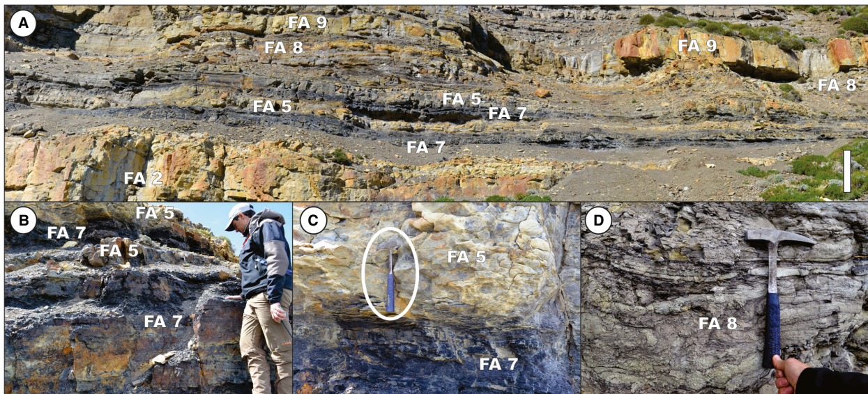
Fig. 6. Coastal plain deposits. A, general view of the coastal plain deposits showing the tabular coals and mudstones (FA 7) at the base, interbedded with lobe-shaped bodies (FA 5), and heterolithic deposits (FA 8) towards the top (scale bar = 5 m). B, C, detail of the tabular coals and the lobe-shaped bodies. D, close-up view of the heterolithic deposits. Hammer: 35 cm.
