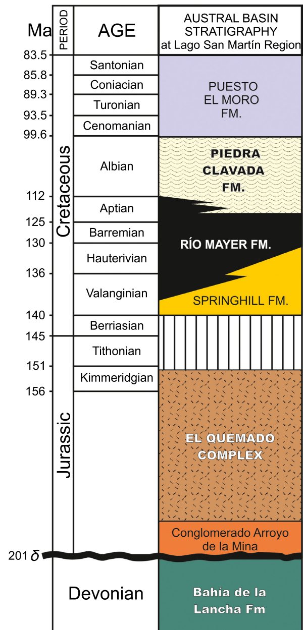
Fig. 2. Stratigraphical chart of the Austral Basin (Argentina) in the study area (Arbe 2002; Richiano et al. 2012; Varela et al. 2012). \delta : discordance.
