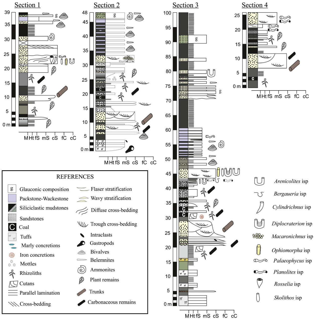
Fig. 3. Sedimentary logs from the Springhill Formation at Lago San Martín region. M: mudstone; Ht: heterolithics; fS: fine-grained sandstone; mS: medium-grained sandstone; cS: coarse-grained sandstone; fC: fine-grained conglomerate; cC: coarse-grained conglomerate (see location in Figures 1B, D).
