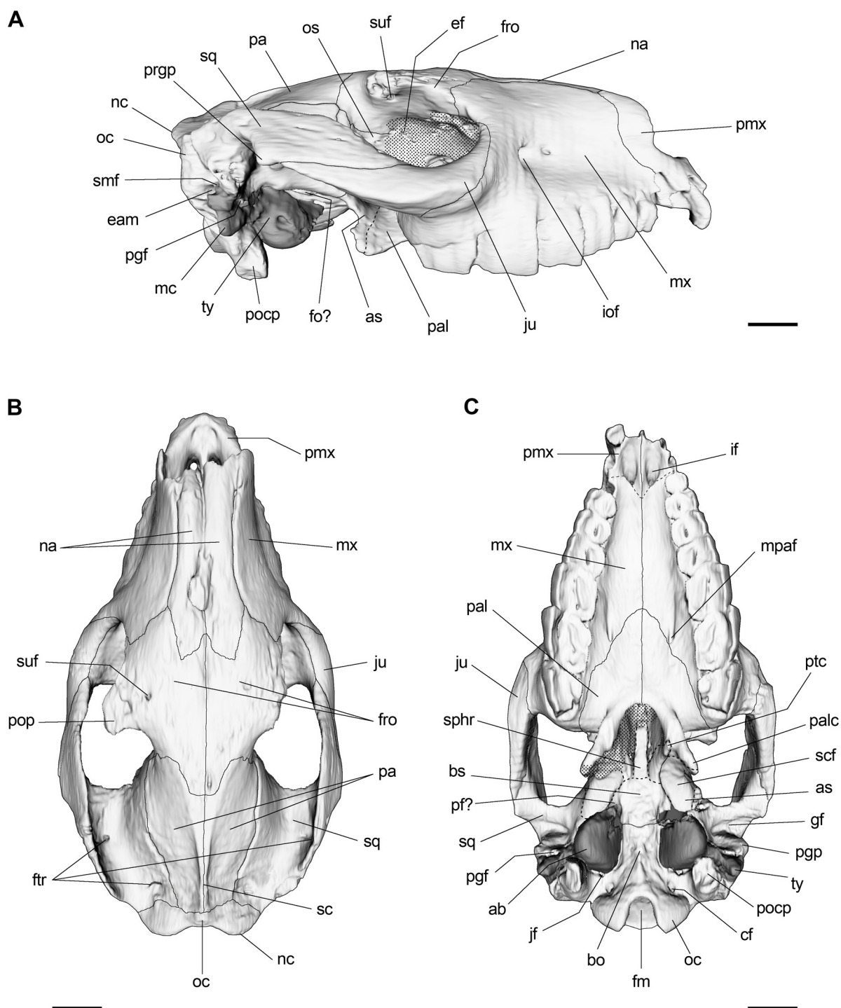
Fig 2. 3D reconstruction of the skull of R. equinus (MPEF-PV 695). (A) Lateral view. (B) Dorsal view. (C) Ventral view. Anatomical abbreviations: ab, auditory bulla; as, alisphenoid; bo, basioccipital; bs, basisphenoid; cf, condylar foramen; eam, external auditory meatus; ef, ethmoidal foramen; fm, foramen magnum; fo, foramen ovale; fro, frontal; ftr, foramina of temporal region; gf, glenoid fossa; if, incisive foramen; iof, infraorbital foramen; jf, jugular foramen; ju, jugal; mc, meatal crest; mpaf, major palatine foramen; mx, maxilla; na, nasal; nc, nuchal crest; oc, occipital; occ, occipital condyle; os, orbitosphenoid; pa, parietal; pal, palatine; palc, palatine crest; pf, piriform fenestra; pgf, postglenoid foramen; pgp, postglenoid process; pmx, premaxilla; pocp, paraoccipital process; pop, postorbital process; prgp, preglenoid process; ptc, pterygoid crest; sc, sagittal crest; scf, scaphoid fossa; smf, suprameatal foramen; sphr, sphenoidal rostrum; sq, squamosal; styf, stylomastoid foramen; suf, supraorbital foramen; ty, tympanic. Scale bar equals 2 cm.
