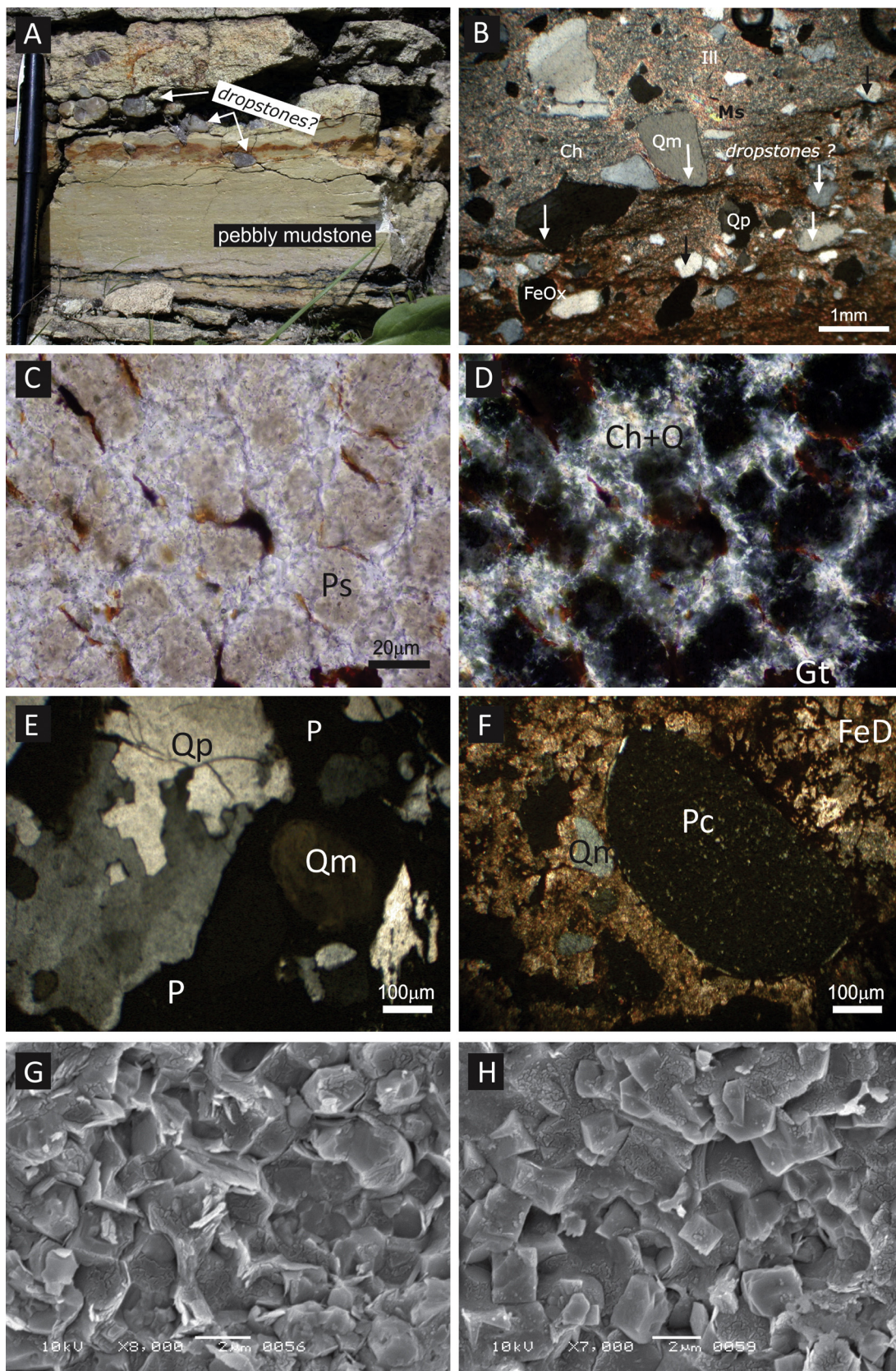
Fig. 5. Petrographic and SEM microphotographs from the VMF phosphate level. (A) and (B) Laminated mudstone with dropstones (modified from Gómez-Peral et al., 2011); (C) and (D) Spherulitic texture of francolite (MP1) without and with crossed nicols. (E) Quartz grains rounded by phosphatic cement. (F) Rounded phosphatic clast in dolomitic cements. (G) and (H) SEM photos showing fluorapatite crystals (P) with hexagonal and pseudocubic habits (see text for brief explanation).
