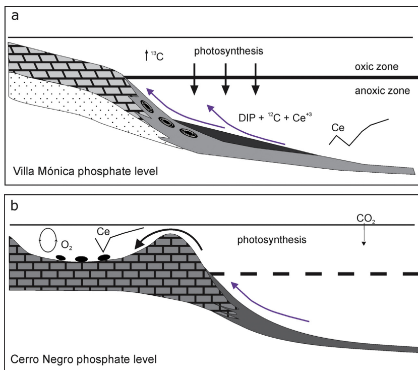
Fig. 11. Schematic representation to explain the genesis of dissolved inorganic phosphorus (DIP), 12 C and Ce enrichment in anoxic water below the redoxcline in a Neoproterozoic stratified ocean basin, modified from Mazumdar et al. (1999). (a) Paleoenvironment of the Villa Mónica Formation with a stratified basin where low Eh and pH conditions facilitate the reductive transformation of Ce 4+ into soluble Ce 3+ , giving a positive Ce anomaly. The redoxcline is a zone that separates the oxic and anoxic parts of the stratified sea basin. (b) Paleoenvironment scheme of the Cerro Negro Formation with well-mixed ocean and normal circulation of oxygen with negative Ce anomalies: organic matter (OM) is quickly remobilized by aerobic oxidation.
