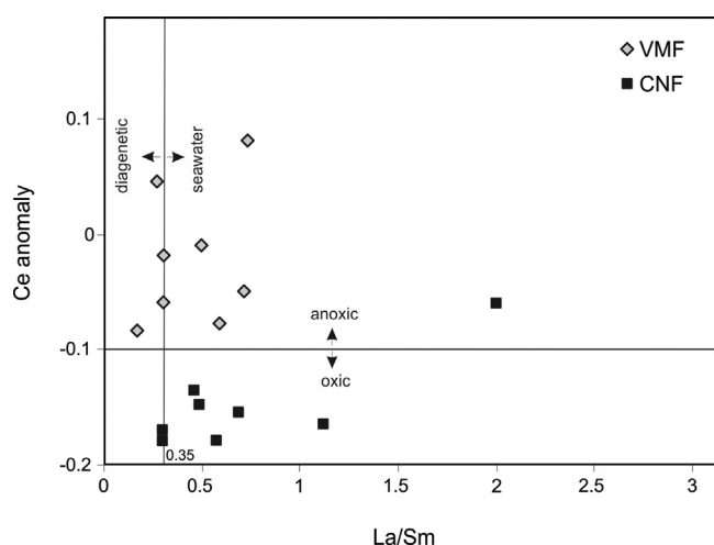
Fig. 8. Crossplot of Ce anomaly vs. \text{La}_N/\text{Sm}_N plotting the ratios of samples of the Villa Mónica and Cerro Negro formations (VMF and CNF).
