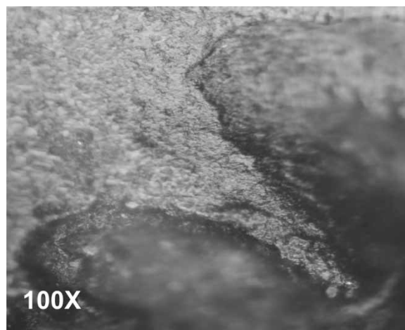
FIGURE 8. Microscars on side edges (bright field illumination—100X).
