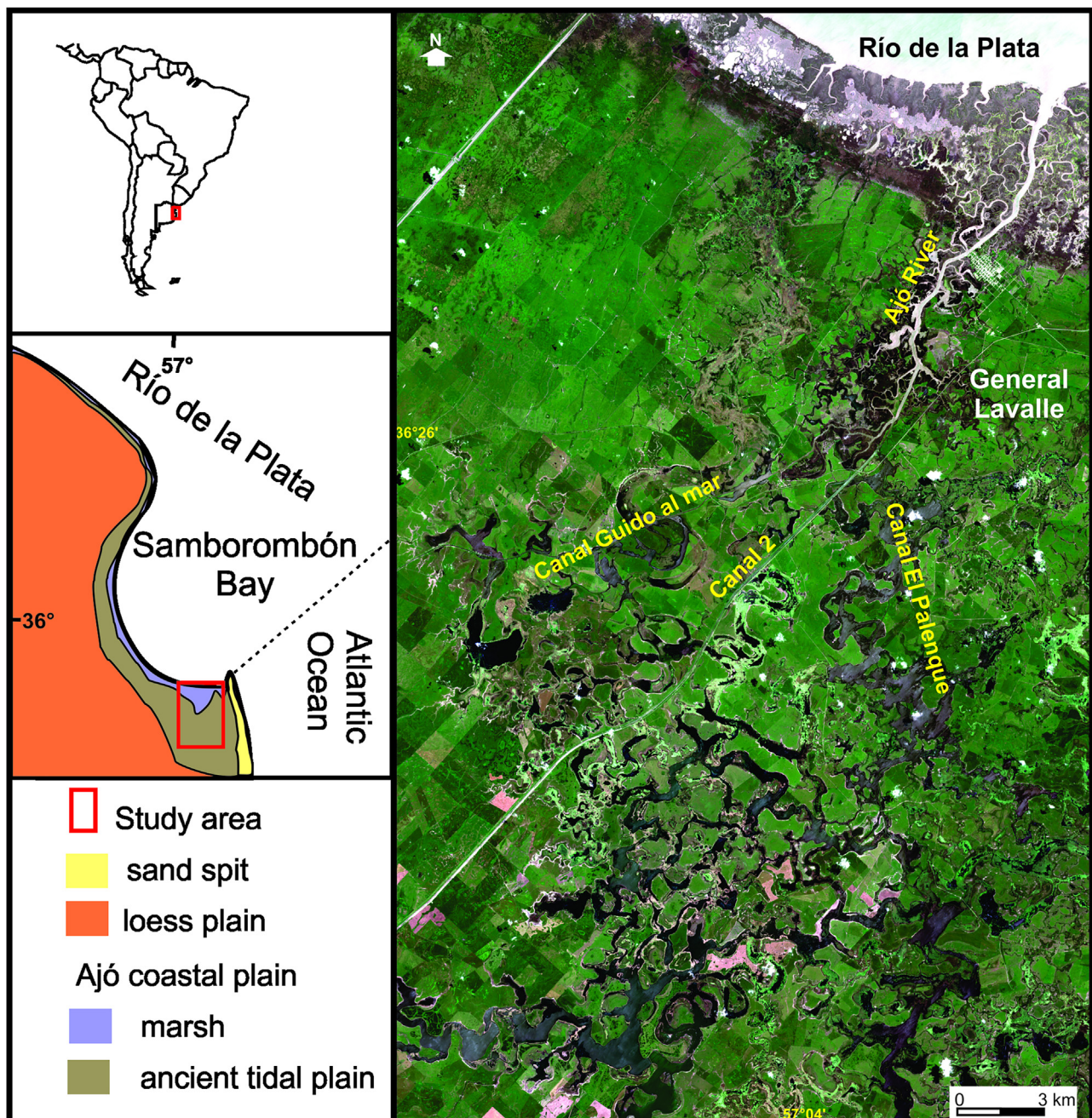
Fig. 1. Location and general setting of the study area. Pseudo-true colour Sentinel-2 image (band combination: R = red, G = green, B = blue).
