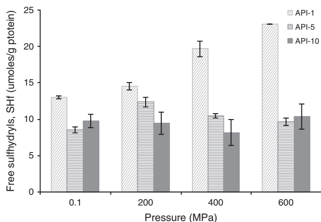
Fig. 4. Free sulphydryl (SH f ) concentration of amaranth protein isolates at 1% w/v (API-1), 5% w/v (API-5) and 10% w/v (API-10) in either native state (0.1 MPa) or after high pressure treatment (200, 400 and 600 MPa).
