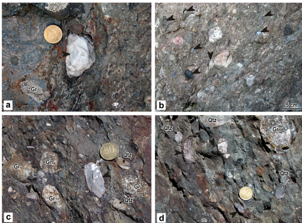
Figure 5. a to d , Diamictites of the Late Carboniferous Sauce Grande Formation from Sierras Australes of Buenos Aires. Massive to thinly laminated grey to white limestone clasts are indicated by arrows. a and b come from diamictite of the locality SV-1; c and d from conglomerate of the SV-2. Other clasts = Gr: granitoid, Gn: gneiss, Qtz: quartzite, diameter of coins: 2.5 cm. This figure is available in colour online at wileyonlinelibrary.com/journal/gj
