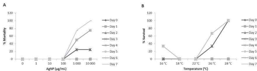
Figure 6. Mortality of P. perlatius exposed to various concentrations of AgNP (A) and various temperatures (B).
