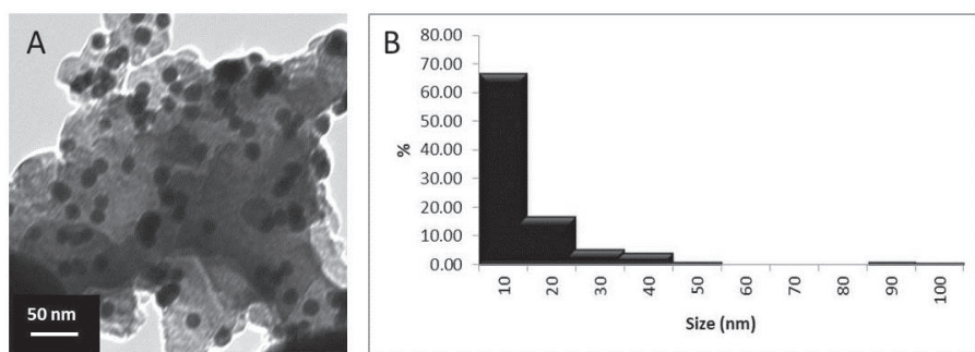
Figure 4. TEM image of dry AgNP (left) with the corresponding particle size distribution (right).
