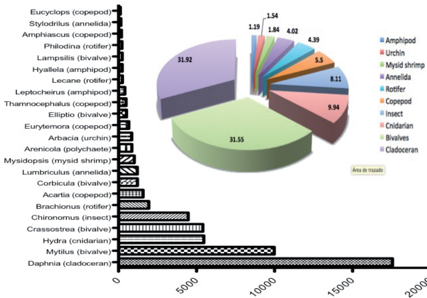
Figure 3. Number of publications for the groups described in the text. The databases consulted were Elsevier ( www.sciencedirect.com ), Springer ( www.link.springer.com ), and Wiley Online Library ( http://onlinelibrary.wiley.com ). Query terms were the genera name and the word “toxicity”. Pie chart data represent percentages based on published material.
