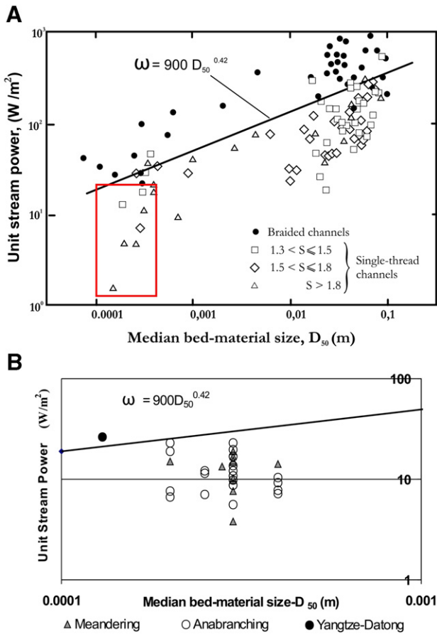
Fig. 12. A) Van den Berg (1995) diagram of channel pattern in relation to grain size and specific stream power. The square identifies the large rivers. B) Enlarged area of Fig. 5A.
