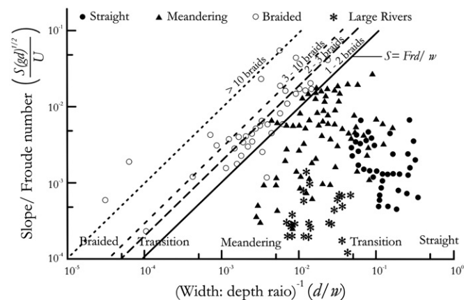
Fig. 13. Parker's (1976) diagram to discriminate straight, meandering, and braided rivers. The degree of braiding is defined in terms of slope/Froude number and d/w ratios.
