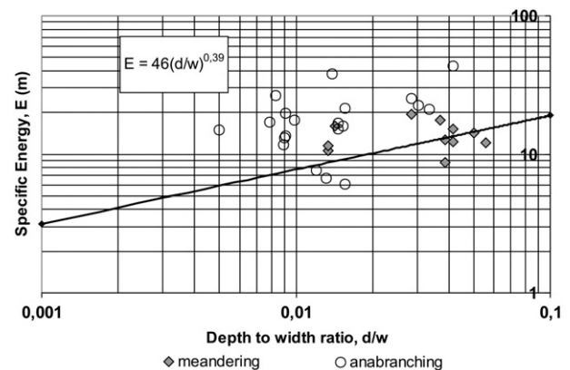
Fig. 14. Large rivers shown by plotting specific energy in relation to depth:width ratio as proposed by Richardson and Thorne (2001). The curve indicates the threshold between single-thread flows and multi-thread flows as found in the Brahmaputra River.
