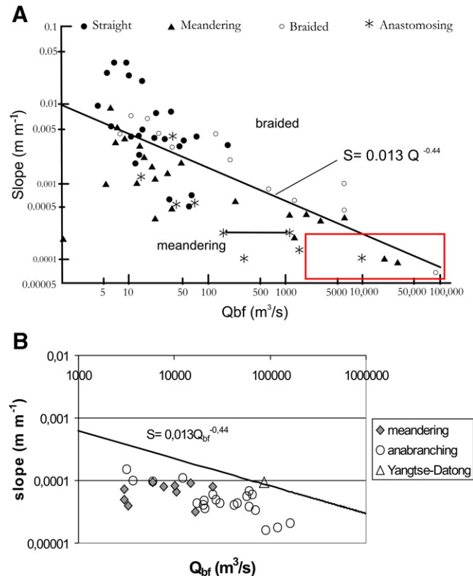
Fig. 10. A) The Leopold and Wolman (1957) slope/bankfull discharge diagram to discriminate channel patterns, including the plot of anabranching rivers by Knighton and Nanson (1993). The squared area indicates the location of the large rivers plotted in Fig. 5B. B) enlarged area of the diagram of Leopold and Wolman.
