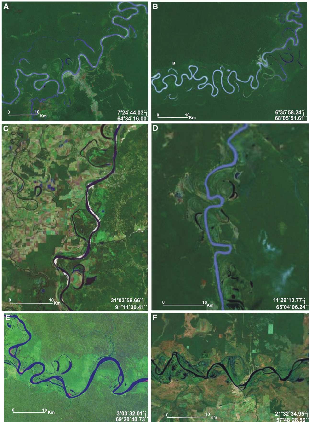
Fig. 4. Meandering rivers. A) Purus River at Labrea ( Q_{\text{mean}} = 5521 \text{ m}^3/\text{s} ); B) Jurua River at Santo Dumont ( Q_{\text{mean}} = 3980 \text{ m}^3/\text{s} ); C) Mississippi at Vicksburg ( Q_{\text{mean}} = 16,660 \text{ m}^3/\text{s} ); D) Mamoré River upstream of Guajara Mirim ( Q_{\text{mean}} = 8154 \text{ m}^3/\text{s} ); E) Iça River at Ipiranga Novo ( Q_{\text{mean}} = 7188 \text{ m}^3/\text{s} ); F) Paraguay River at Porto Murtinho ( Q_{\text{mean}} = 2376 \text{ m}^3/\text{s} ).
