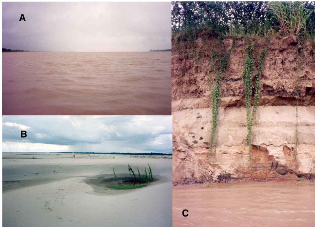
Fig. 6. The Solimões River at Manacapuru area. A) The main channel, B) large sand bar at low water stage, C) exposure of channel cutbank, ~7 m high, at the head of Marchantaria Island.
