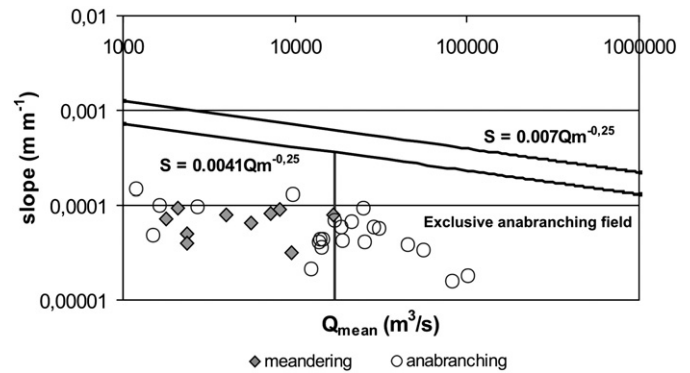
Fig. 11. Lane (1957) slope/mean annual discharge diagram to discriminate channel patterns. The figure shows an enlarged area where large rivers plot.
