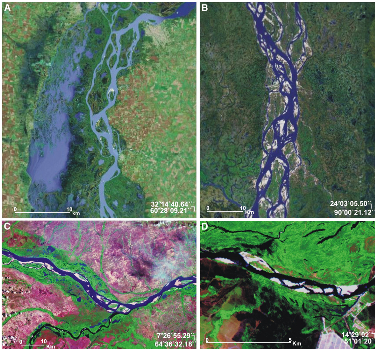
Fig. 7. Anabranching rivers with tendency towards braided pattern. A) lower Parana River downstream of Santa Fe (downstream Villa Urquiza gauge station) ( Q_{\text{mean}} = 16,400 m 3 /s); B) Brahmaputra at Baharudabad ( Q_{\text{mean}} = 21,261 m 3 /s); C) Orinoco River at Musinacio ( Q_{\text{mean}} = 28,723 m 3 /s); D) Araguaia River at Luiz Alves ( Q_{\text{mean}} = 3700 m 3 /s).
