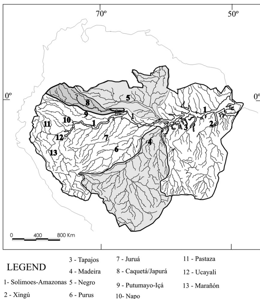
Fig. 2. Main sub-basins of the Amazon drainage basin. The Madeira River, Negro River and Japura River basins (dashed areas) complete the list of the ten largest rivers (Fig. 1).
