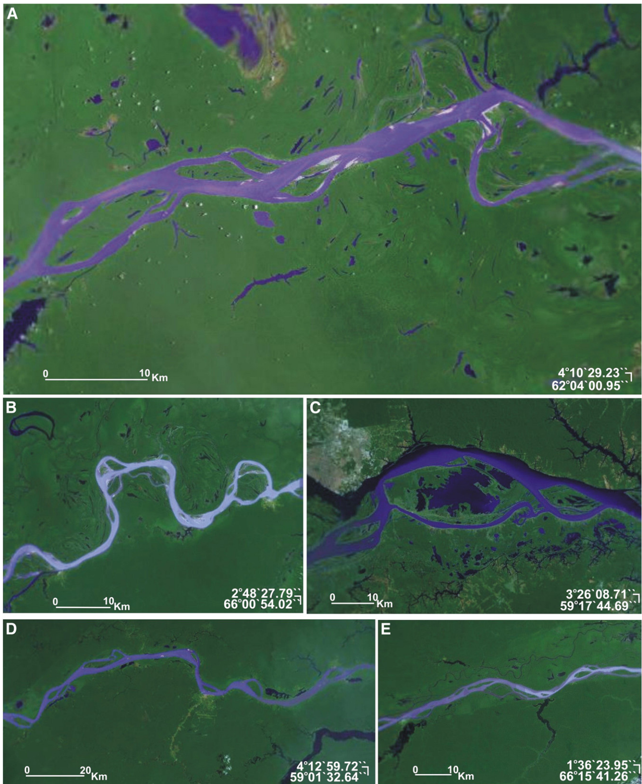
Fig. 5. Low sinuosity anabranching patterns. A) Solimões–Amazon immediately downstream of Itapeua; B) Solimões–Amazon at Fonte Boa downstream of Santo Antonio do Iça ( Q_{\text{mean}} \sim 55,600 \text{ m}^3/\text{s} ); C) Amazon at Careiro Island, Jatuarana station ( Q_{\text{mean}} = 123,680 \text{ m}^3/\text{s} ); D) Madeira River at Fazenda Vista Alegre ( Q_{\text{mean}} = 31,000 \text{ m}^3/\text{s} ); E) Japura River at Acanauí ( Q_{\text{mean}} = 14,333 \text{ m}^3/\text{s} ).
