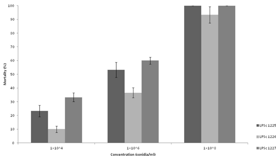
Fig. 1. Cumulative mortality (%) \pm SD of third-instar Schistocerca cancellata nymphs within 10 days after inoculation with 1 \times 10^4 ; 1 \times 10^6 and 1 \times 10^8 conidia/ml of Beauveria bassiana (LPSc 1225; LPSc 1226 and LPSc 1227).
