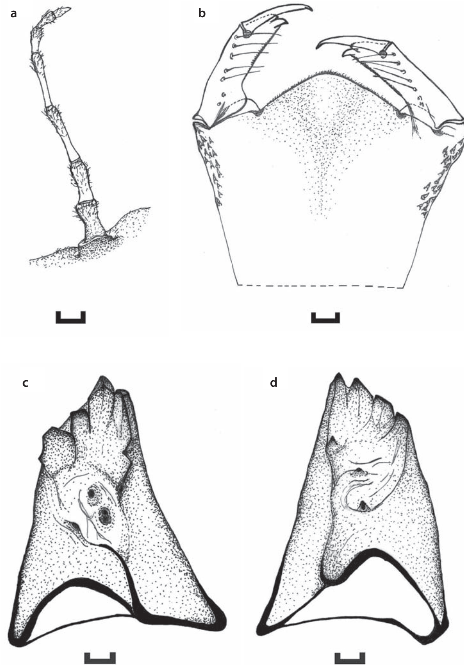
Figure 1: Final stadium larva of Mecistogaster amalia — (a) antenna; (b) prementum, dorsal view; (c) left mandible, internal view; (d) right mandible, internal view. Scale lines: 0.5 mm.
