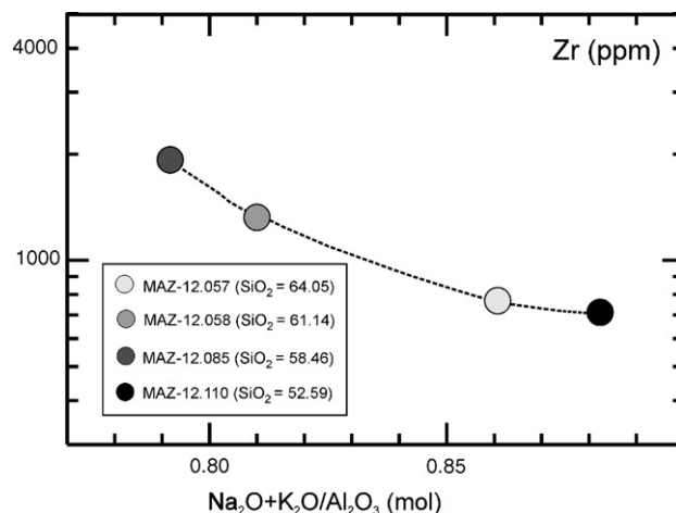
Fig. 5. Plot of \text{Zr} vs. (\text{Na}_2\text{O} + \text{K}_2\text{O})/\text{Al}_2\text{O}_3 (mol) for the syenitic suite of Sierra de Maz.
