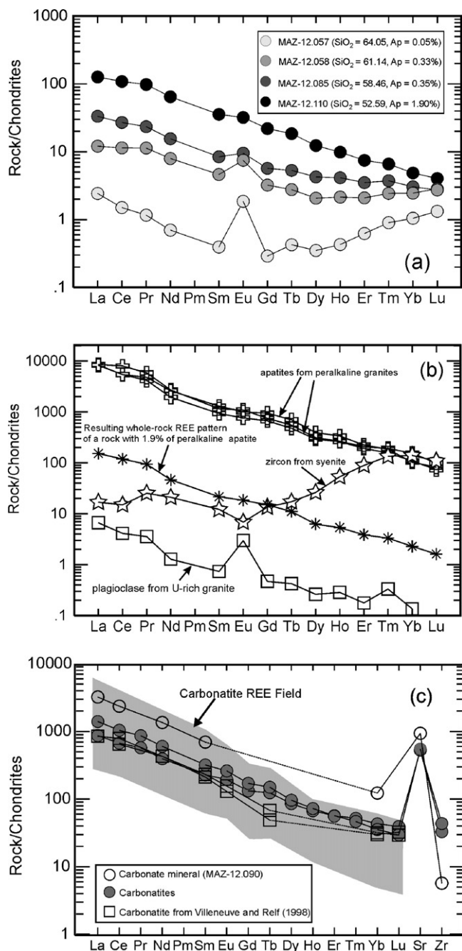
Fig. 7. (a) Chondrite-normalized REE abundances of the syenitic suite of the Sierra de Maz complex. (b) Selected REE patterns of apatite, zircon and plagioclase from alkaline rocks and U-rich granites, from Bea (1996). Note that a modelled REE pattern for a rock with 1.9% of normative apatite closely resembles the pattern of the least evolved member of the syenitic suite (sample MAZ-12.110). (c) REE, Sr and Zr plot of two silico-carbonatite samples from the Sierra de Maz complex. The open circle represents a single homogeneous crystal of carbonate separated from the carbonatite. The general carbonatite field is taken from 13 samples reported by Nelson et al. (1988), whereas open squares are carbonatites reported by Villeneuve and Relf (1998). Data are normalized to chondritic values of Nakamura (1974); other normalizing data from Boynton (1984) for Tb, Ho, Tm, and Sr and Thompson (1982) for Zr.
