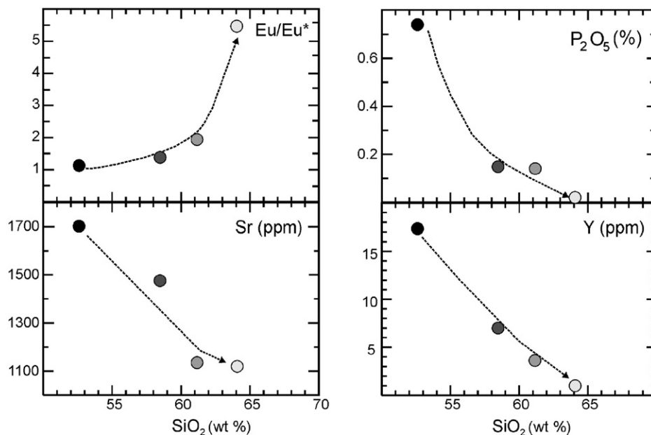
Fig. 6. \text{Eu}/\text{Eu}^* , \text{P}_2\text{O}_5 , Sr and Y vs. \text{SiO}_2 wt.% for the syenitic suite of Sierra de Maz.
