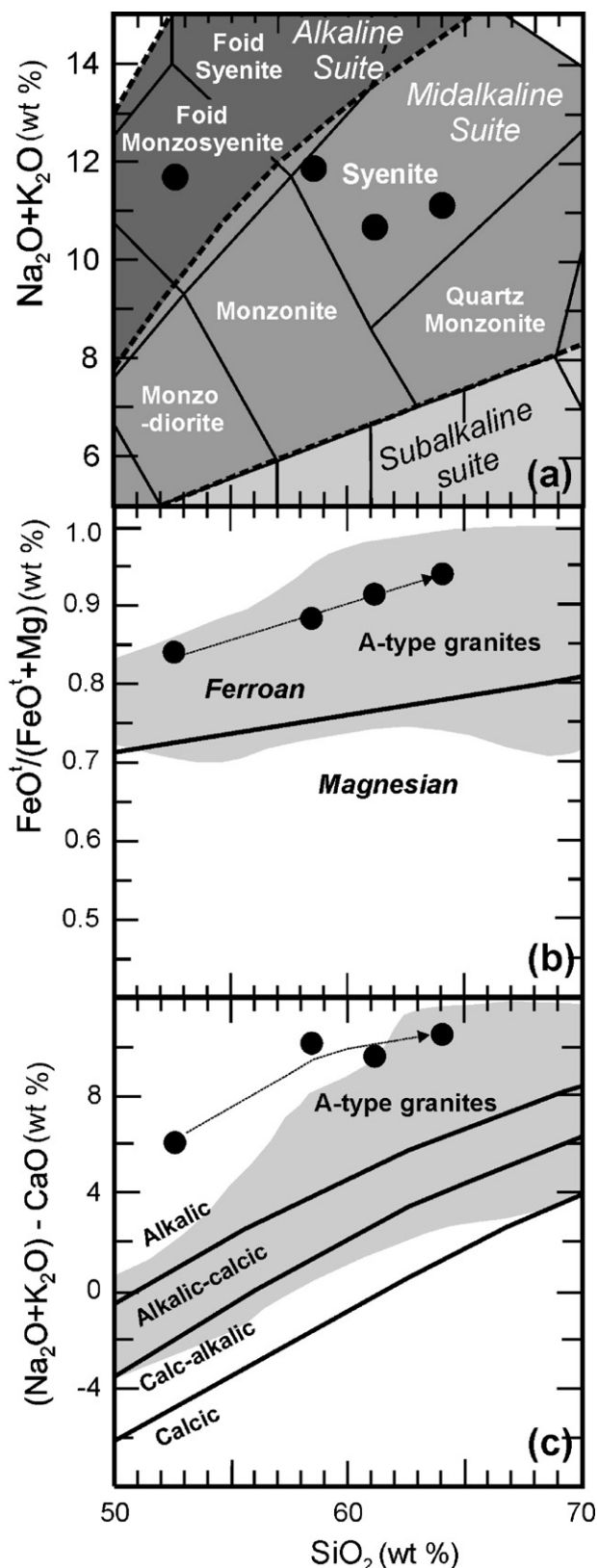
Fig. 4. (a) Nomenclature of plutonic rocks and different suite lineages, after Middlemost (1997). (b) \text{FeO}^1/(\text{FeO}^1 + \text{MgO}) vs. \text{SiO}_2 wt.%, showing the Frost et al. (2001) boundary between ferroan and magnesian plutonic rocks, as well as the field of A-type granites. (c) Plot of \text{Na}_2\text{O} + \text{K}_2\text{O} - \text{CaO} against \text{SiO}_2 wt.% for the syenitic suite of Sierra de Maz. Limits for the rock series and field of A-type granites are from Frost et al. (2001).
