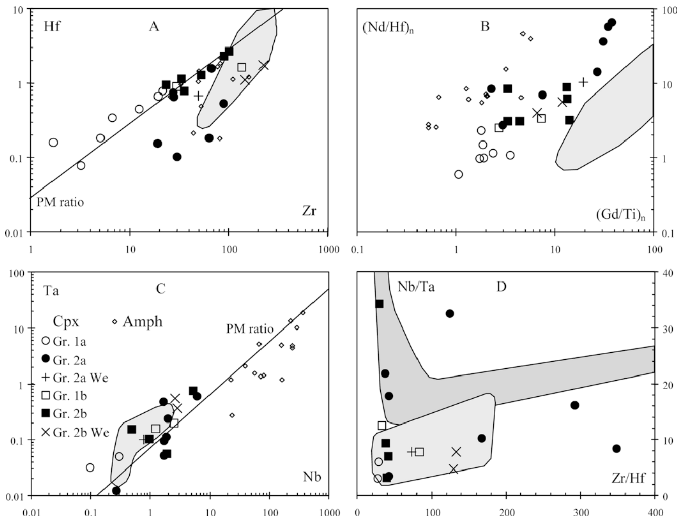
Fig. 8a–d Relationships of selected elements (ppm) and element ratios in clinopyroxenes and amphiboles. a Zr–Hf correlation, b Gd_n/Ti_n – Nd_n/Hf_n relationship, c Nb–Ta (ppm) correlation, d variation of Nb/Ta vs. Zr/Hf. Composition of the Australian clinopyroxenes (Yaxley and Kamenetsky 1999) is reported as a light-shaded field. Amphiboles in d are represented by the dark-shaded field
