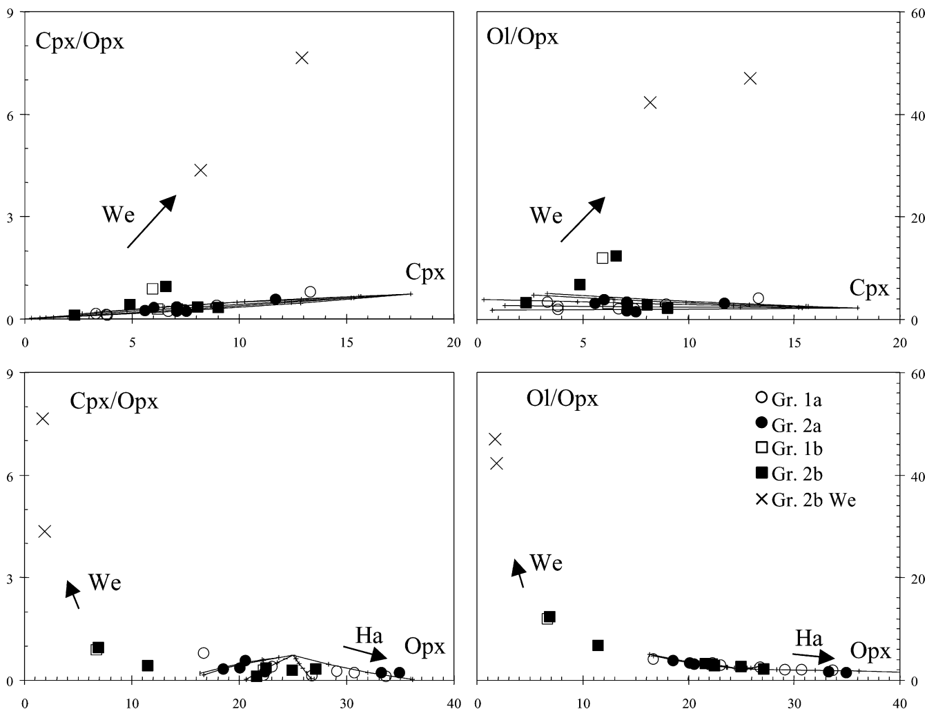
Fig. 2 Variation of the modal ratios \text{cpx/olpx} and \text{ol/olpx} versus modal \text{cpx} and \text{olpx} . Thin lines are model variation trends induced by anhydrous (Baker and Stolper 1994; Kinzler 1997, at 1.9 GPa) and hydrous (Hirose and Kawamoto 1995; Gaetani and Grove 1998, at 1.2 GPa) melting on a mantle having the mode reported by Johnson et al. (1990). The arrows are qualitative vectors of reactions dissolving olivine and forming \text{opx} (Ha harzburgite trend) and dissolving \text{opx} and forming \text{ol} and \text{cpx} (We wehrlite trend).
