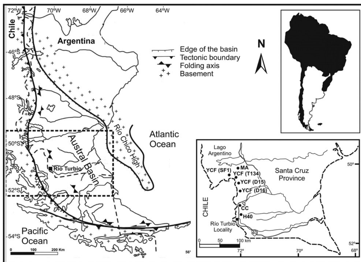
Figure 1. Map of southern Patagonia showing the extent of the Austral Basin. The inset map shows southern Santa Cruz Province and the location of the upper member of the Río Turbio Formation at: YCF Cores (cores, 50° 45' 14" S, 72° 01' 39" W; 50° 56' 21" S, 72° 02' 08" W; 50° 35' 59" S, 72° 13' 40" W); the Cancha Carrera locality (CC) (outcrop sections, 51° 14' 34" S, 72° 15' 26" W); the Highway 40 locality (H40) (outcrop sections, 51° 31' 13" S, 72° 15' 11" W); and the outcrop section of the Man Aike Formation (50° 21' 45" S, 72° 14' 30" W). Modified from Nullo, Panza & Blasco (1999).
