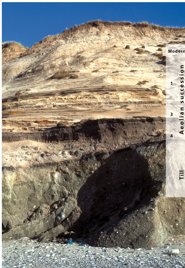
Fig. 15. Coastal cliff section at Lodbjerg, Denmark. A Weichselian till at the base of the section is overlain by 15 to 20 m of aeolian sand with peaty soils (dark horizons). Terminology of aeolian events after Clemmensen et al. (2009).
