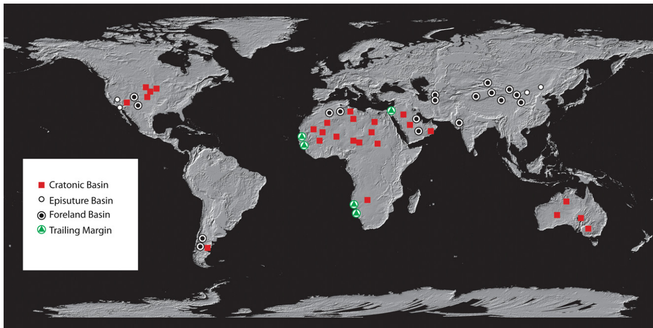
Fig. 10. Tectonic setting of major inland sand seas and dune fields. Tectonic data from Fugro Tellus Sedimentary Basins of the World Map http://www.datapages.com/AssociatedWebsites/GISOpenFiles/FugroTellusSedimentaryBasinsoftheWorldMap.aspx . See also Table S5.
