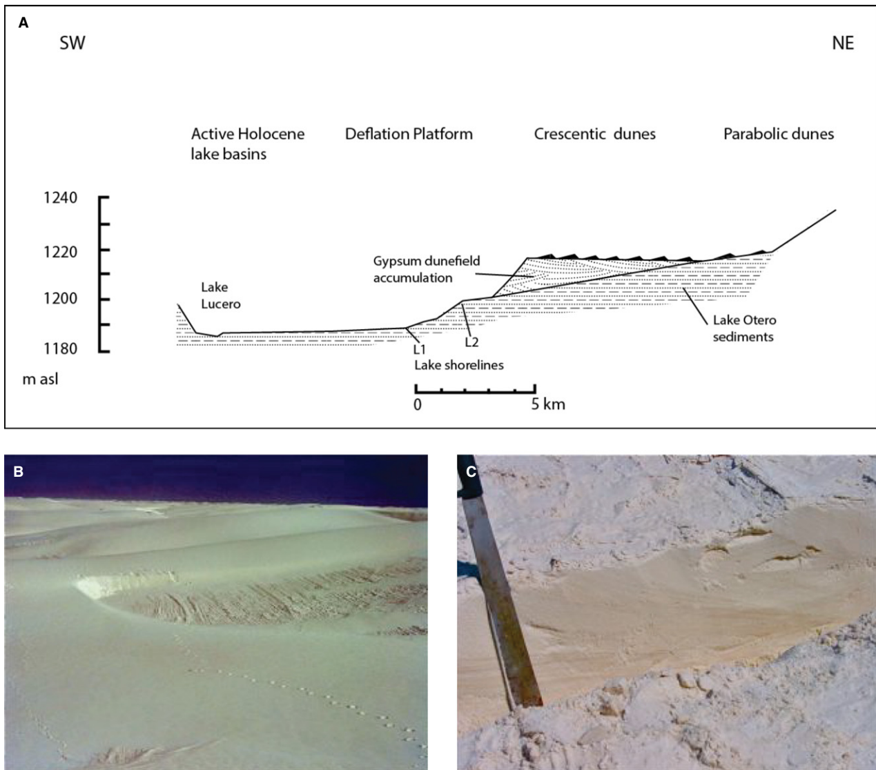
Fig. 11. Example of a wet aeolian system: White Sands, New Mexico, USA: (A) cross-section of dunefield showing relations between aeolian and lacustrine sediments (after Kocurek et al. , 2007); (B) 3 to 5 m high crescentic ridges migrating across the surface of older crescentic dune deposits shown by exposed cross-bedding; (C) trench in an interdune area showing cross-bedded dune structures. Machete is ca 0.6 m long.
