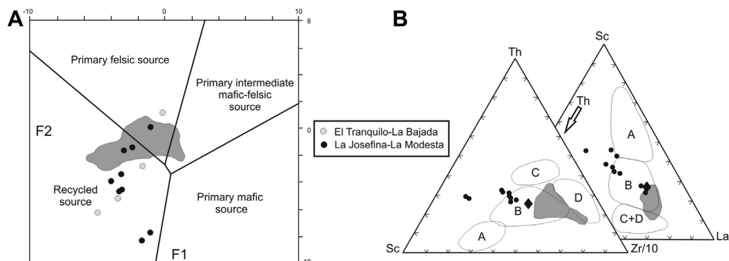
Fig. 7. A: Major element discrimination scheme for the La Modesta Formation samples (excluded those containing calcite). Diagram after Roser and Korsch (1988). Grey field: Bahia La Lancha and Rio Lacteo Formations and Cochrane Unit from Augustsson and Balbhurg (2008). B: La Josefin-La Modesta samples in trace elements ternary diagrams for discrimination between greywackes from different tectonic environments (Bhatia and Crook, 1986). A: Ocean island arc, B: Continental island arc, C: Active continental margin, D: Passive margin. Diamonds: Upper Continental Crust (McLennan, 2001). Grey field: Bahia La Lancha and Rio Lacteo Formations and Cochrane Unit from Augustsson and Balbhurg (2008).
