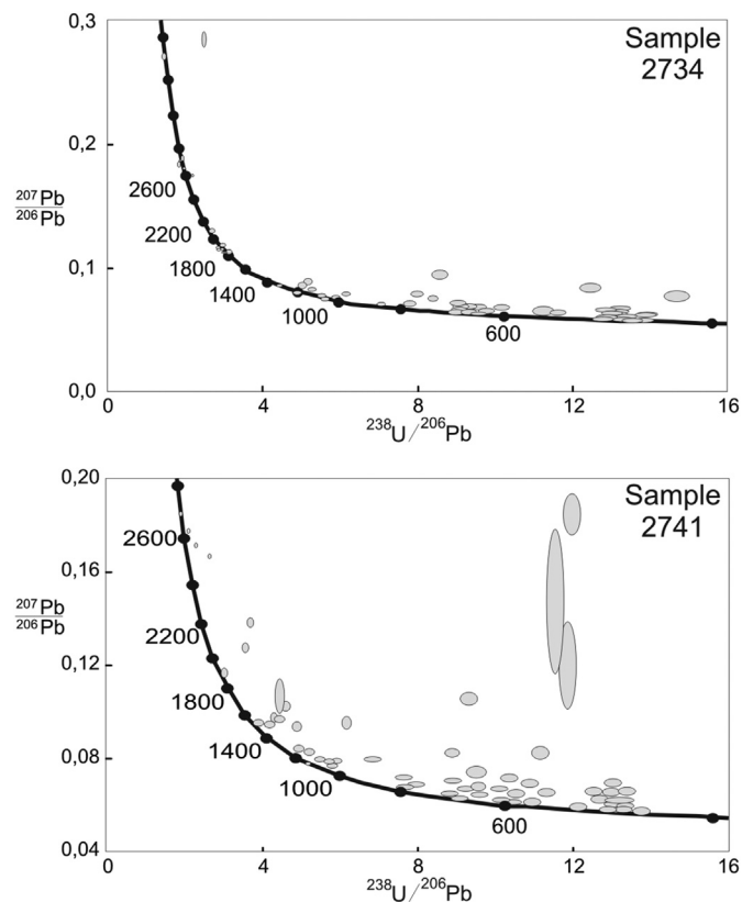
Fig. 4. Tera-Wasserburg U–Pb Concordia diagrams for SHRIMP analyses of zircons from samples 2734 and 2741 of the La Modesta Formation.
