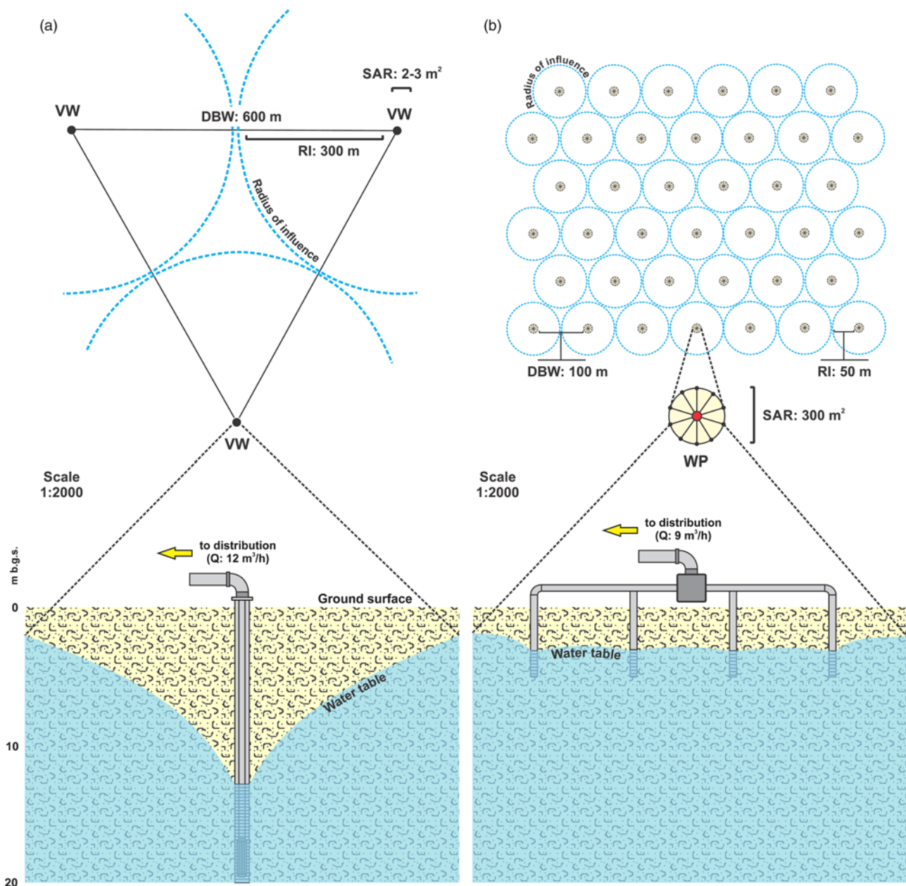
Fig. 2. Spatial distribution for (a) vertical well (VW) and (b) wellpoint (WP). DBW, distance between wells, SAR, surface area required; RI, radius of influence.
